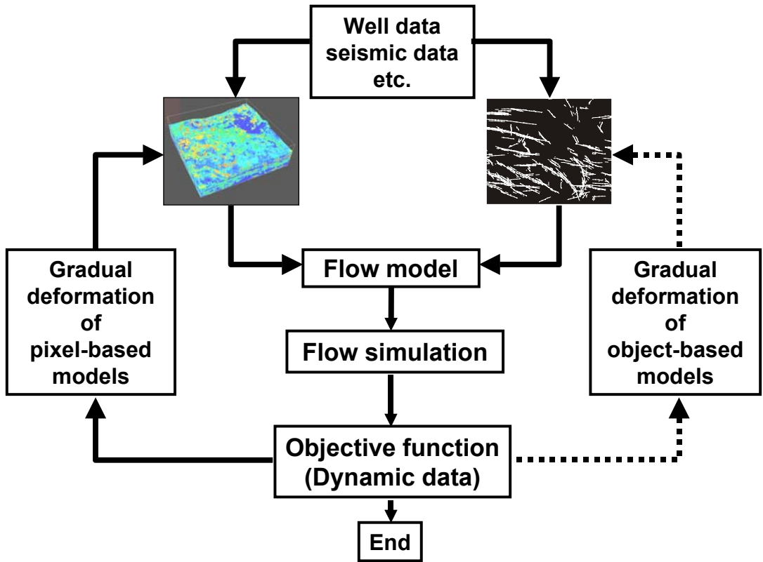
Integrated workflow for history matching of stochastic reservoir models with heterogeneous matrix and fault/fracture network
