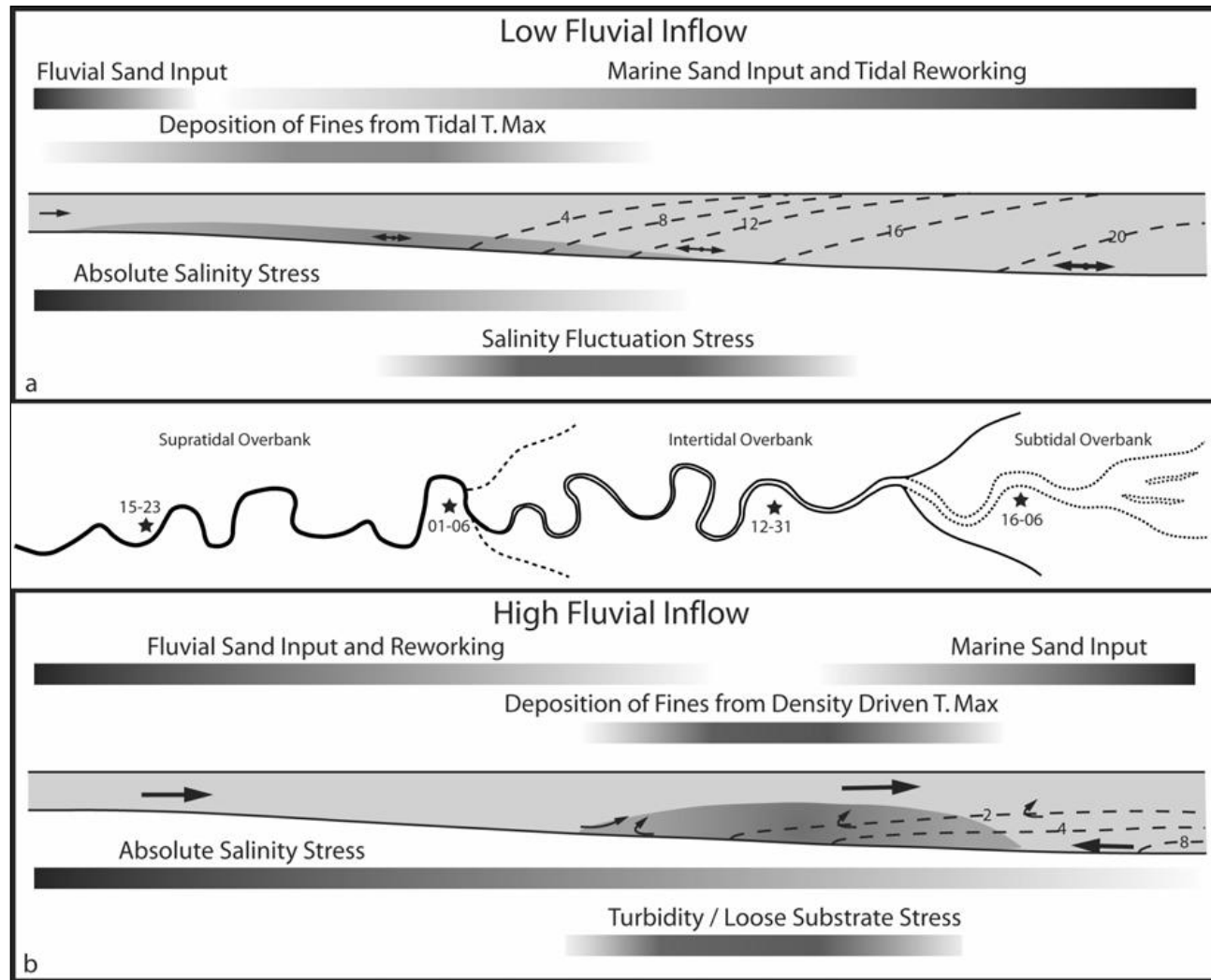
Figure 1. Schematic showing spatial and temporal variation of depositional character within a riverine estuary. a) During periods of low fluvial inflow, tidal processes dominate over fluvial/density circulation processes and the system experiences a deep incursion of brackish water. Deposition of fines is skewed towards the fluvial end and has a laminated tidal character. The marine end of the system experiences tidal reworking with a net landward flux of sediment. b) During periods of high fluvial inflow, fluvial/density circulation processes dominate over tidal processes and brackish water is flushed from much of the system. Deposition of fines is skewed towards the marine end and has a largely structureless character. The fluvial end of the system experiences reworking with a net seaward flux of sediment. T. Max for turbidity maximum.
