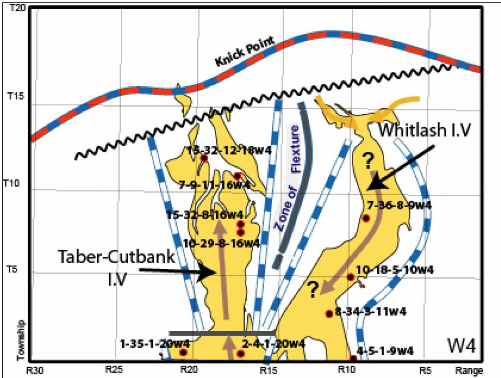
Figure 1. Location map of study wells placed on a palaeogeographic reconstruction taken from Zaitlin et al. (2002).
