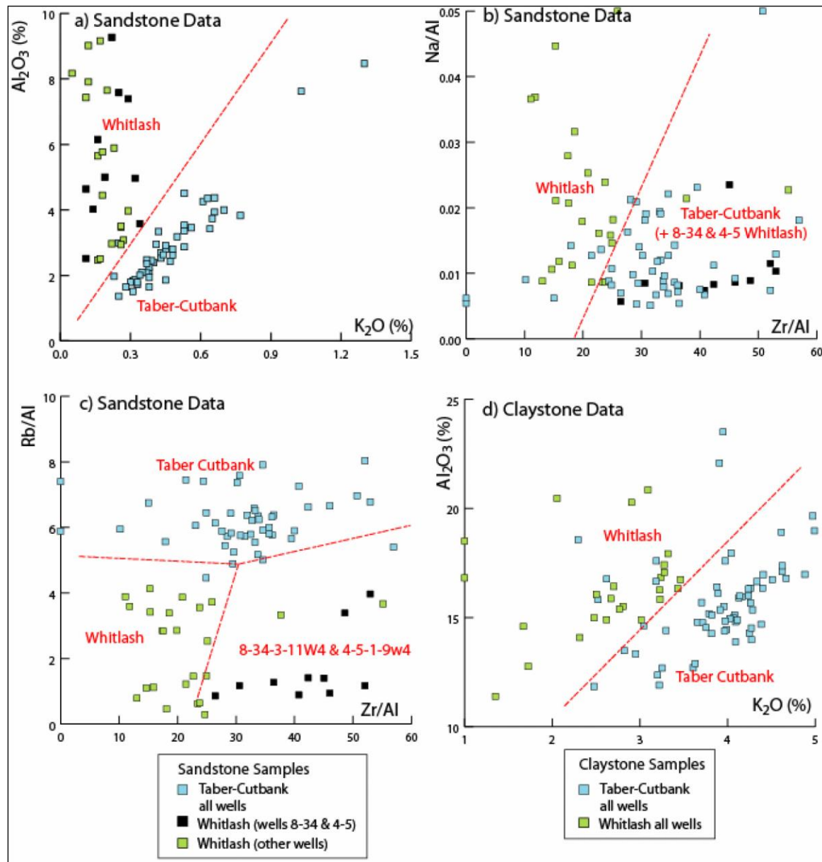
Figure 4. Binary diagrams constructed to demonstrate a-c) differentiation of Whitlash I.V. Horsefly from Taber-Cutbank I.V. Horsefly using sandstone data d) differentiation of Whitlash I.V. Horsefly from Taber-Cutbank I.V. Horsefly using claystone data.
