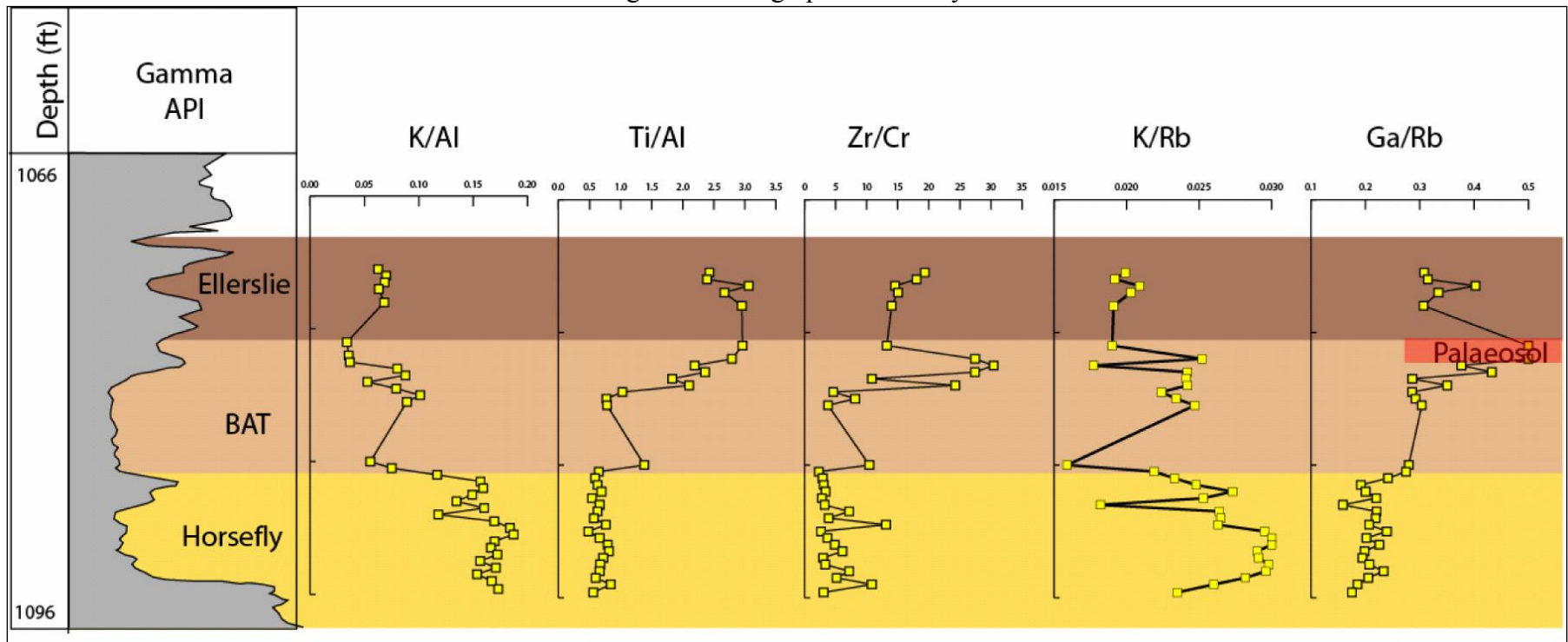
Figure 2. Stratigraphic summary.
