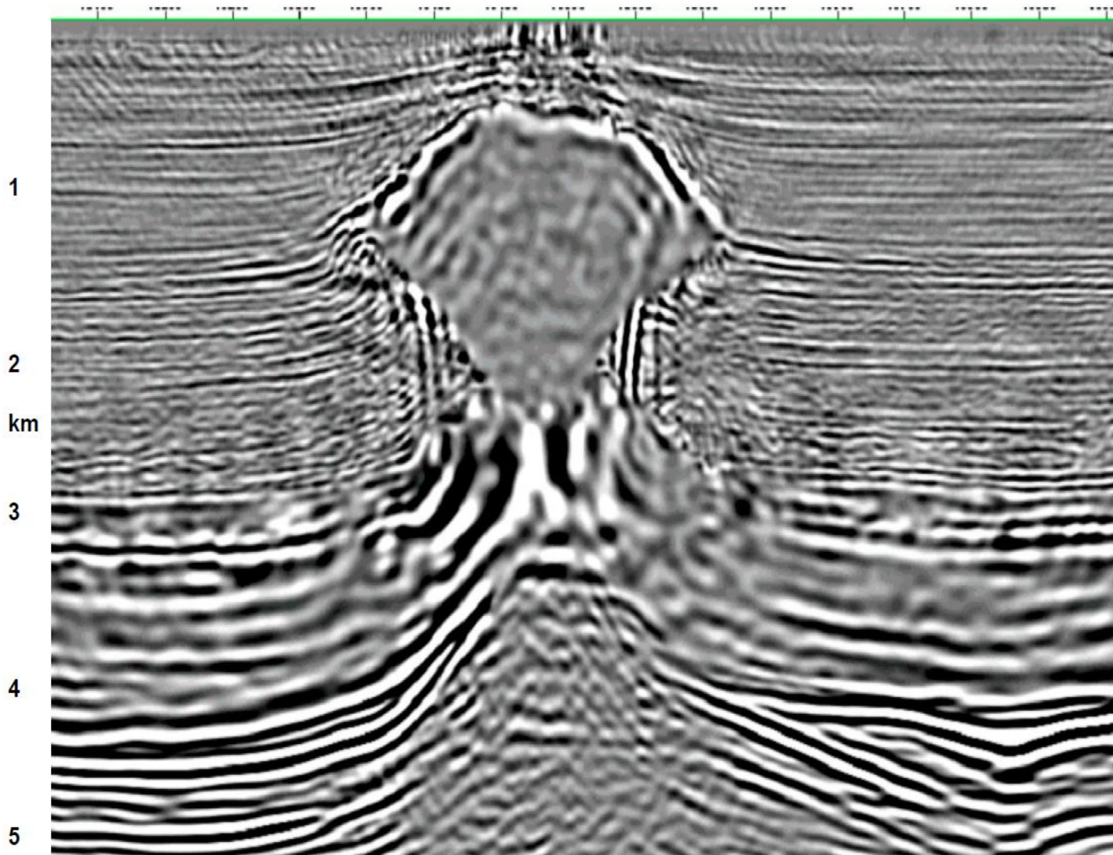
Figure 3. 'Final' production model: Two-Way RTM.
