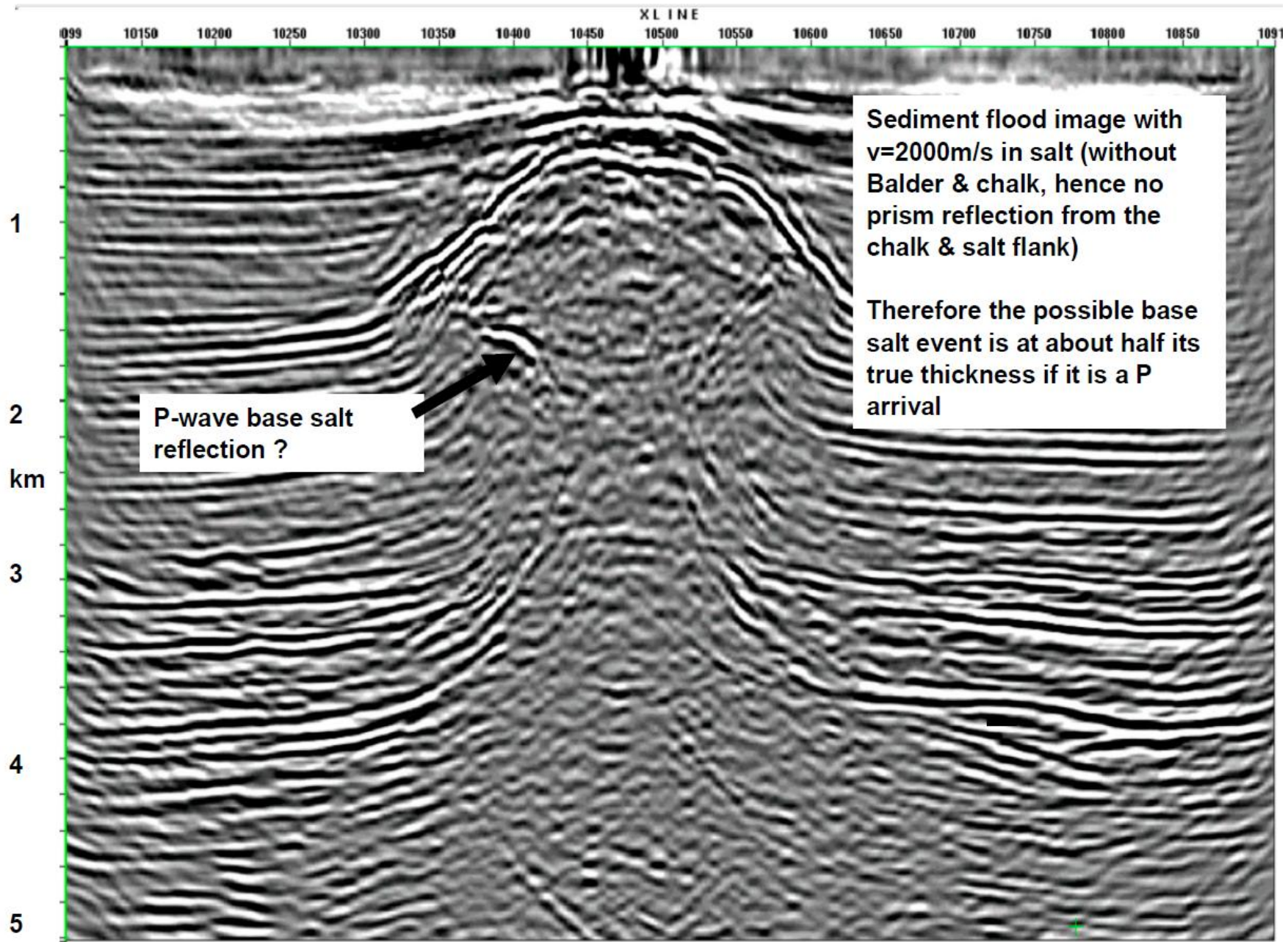
Figure 4. Sediment flood RTM (no chalk thus no double bounce arrivals).
