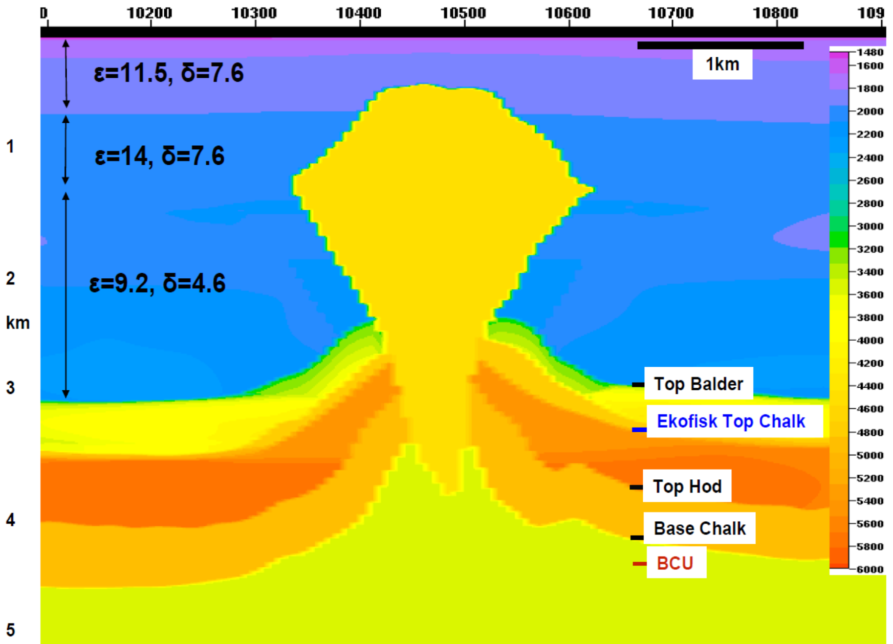
Figure 1. 'Final' production 3D migration velocity field.
