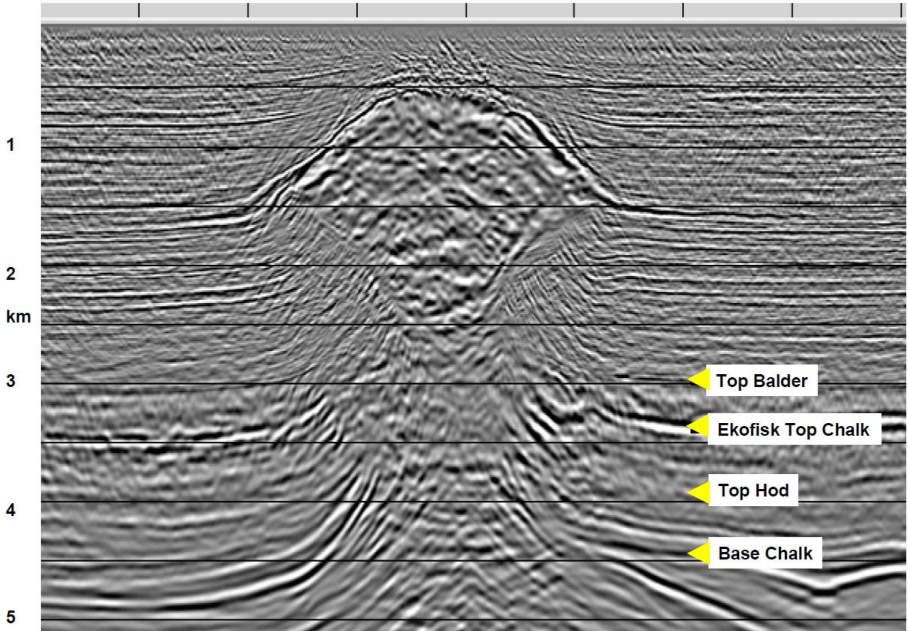
Figure 2. 'Final' production model: One-Way WEM.
