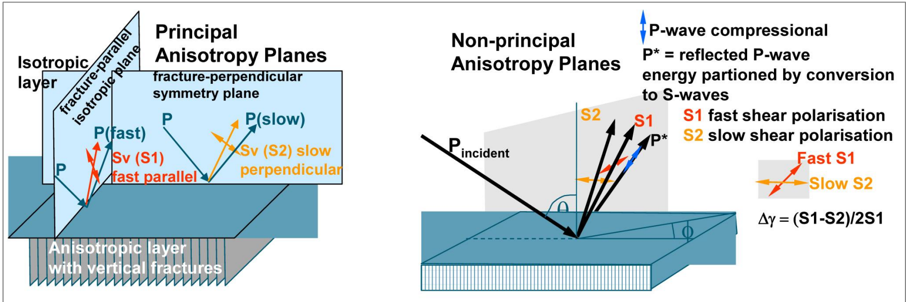
Figure 4. Model of HTI media used in Ruger's 1997 AVAZ P-wave reflection equation showing anisotropic conversion to shear-waves for principal and non-principal planes of symmetry.
