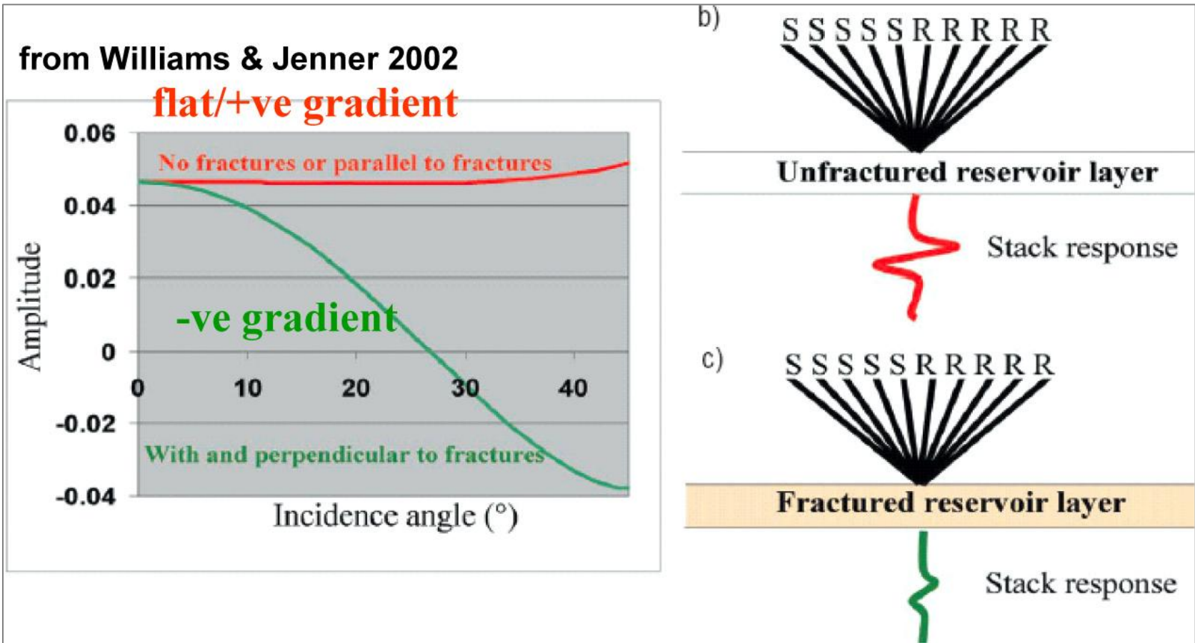
Figure 1. AVAZ variation with stack response: - parallel is strong (flat to +ve gradient); - perpendicular is weak (-ve gradient); a) from Williams and Jenner (2002).
