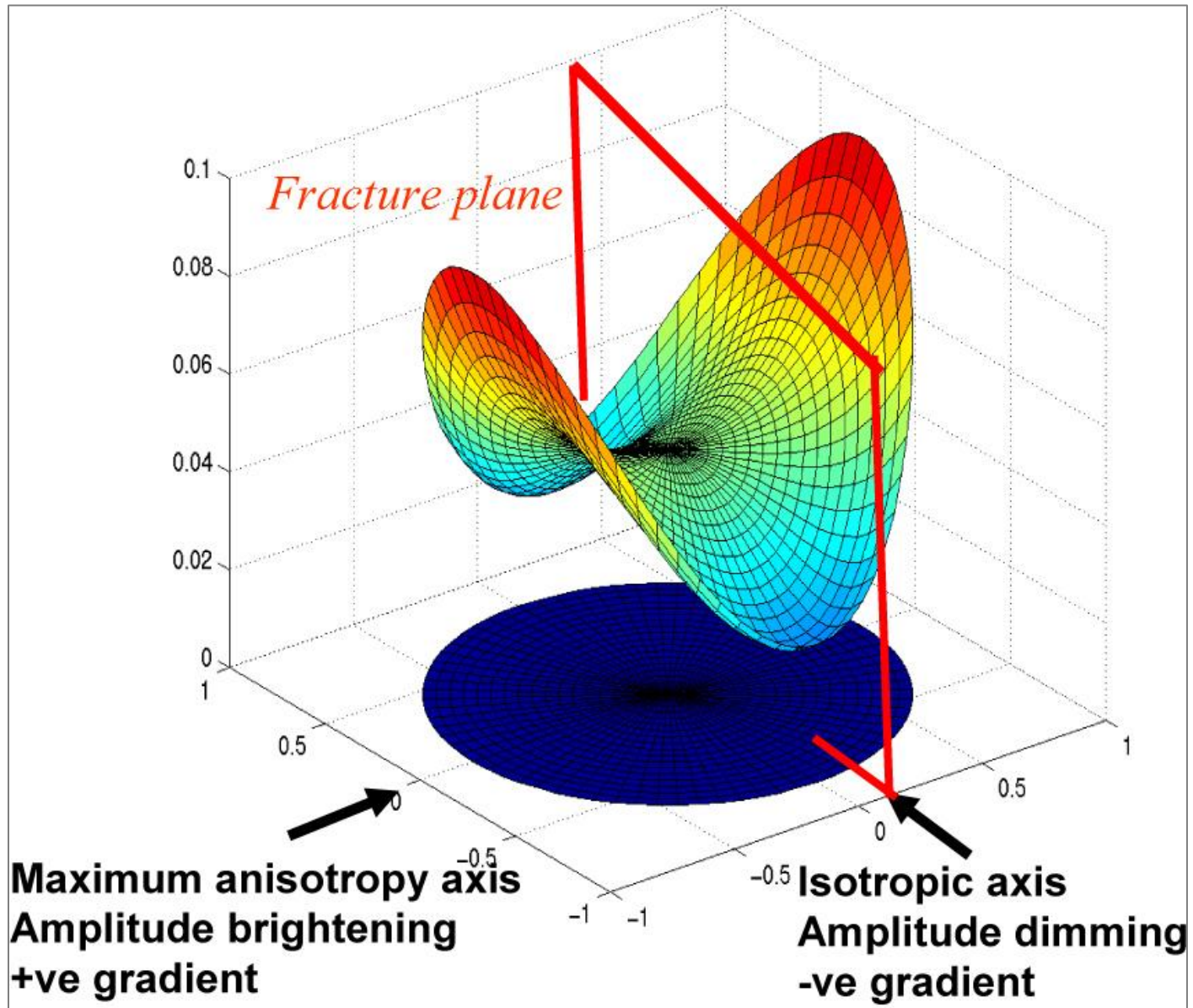
Figure 2. Amplitude variation in HTI medium as advertised by contractor industry. (polar azimuth plots of gradients, modelled from Ruger's AVAZ equation).
