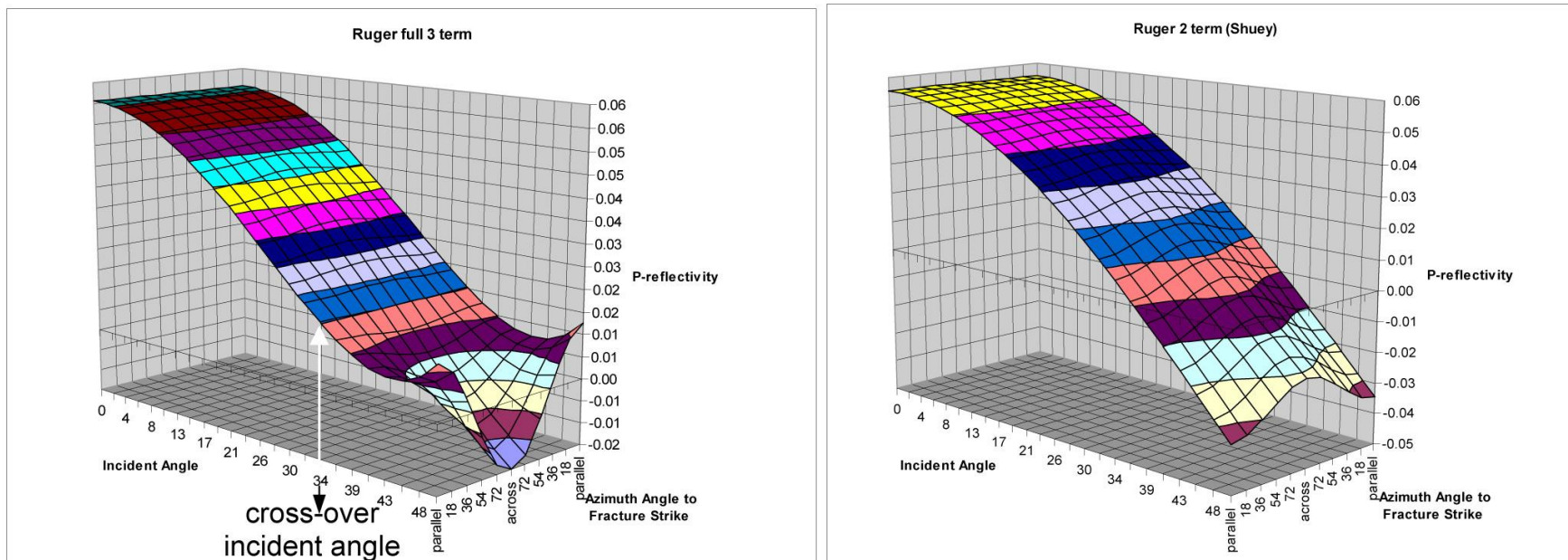
Figure 5. 5a and 5b: 3D displays of Ruger's 3 term vs. 2 term (Shuey, 1985) equation of azimuthal AVO curves.
