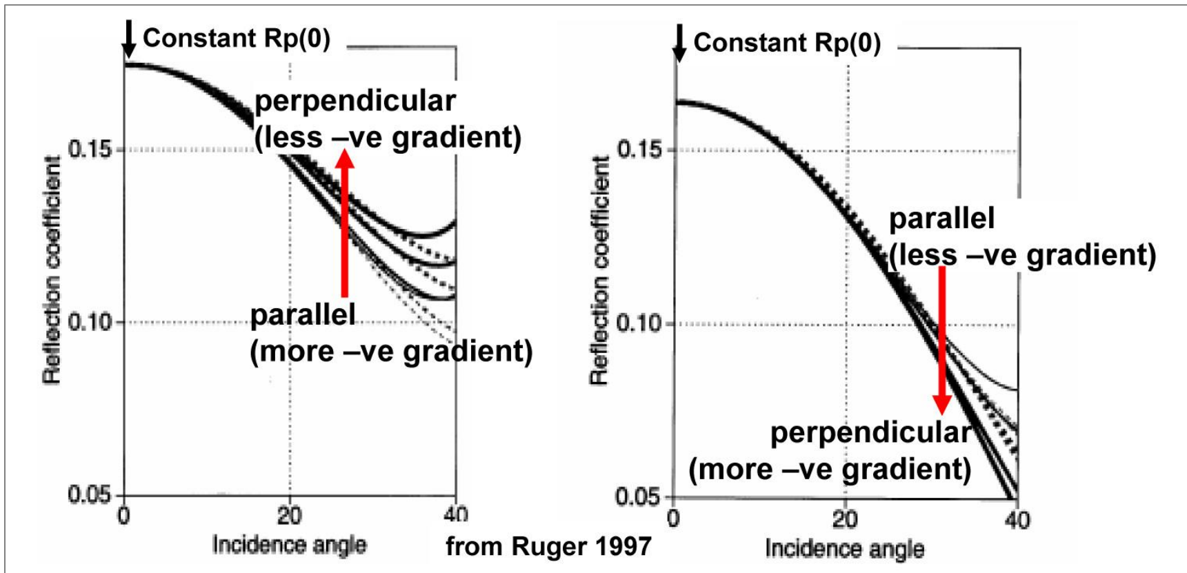
Figure 3. Ruger's (Ruger and Tsvankin, 1997) models based on his linearized 3 term azimuthal AVO gradient equation.
