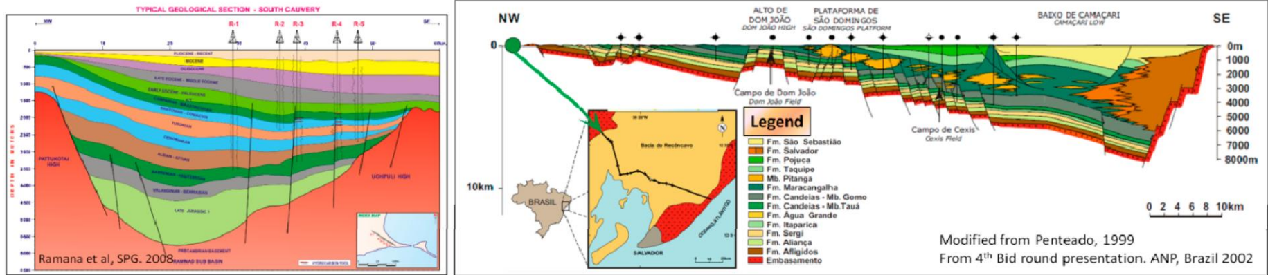
Figure 3a and b. Representative geological sections across the Cauvery Basin, India and the Reconcravo Basin, Brazil. The crowding of successful wells on the gentle flank of the half-grabens indicates higher propensity for hydrocarbons.
