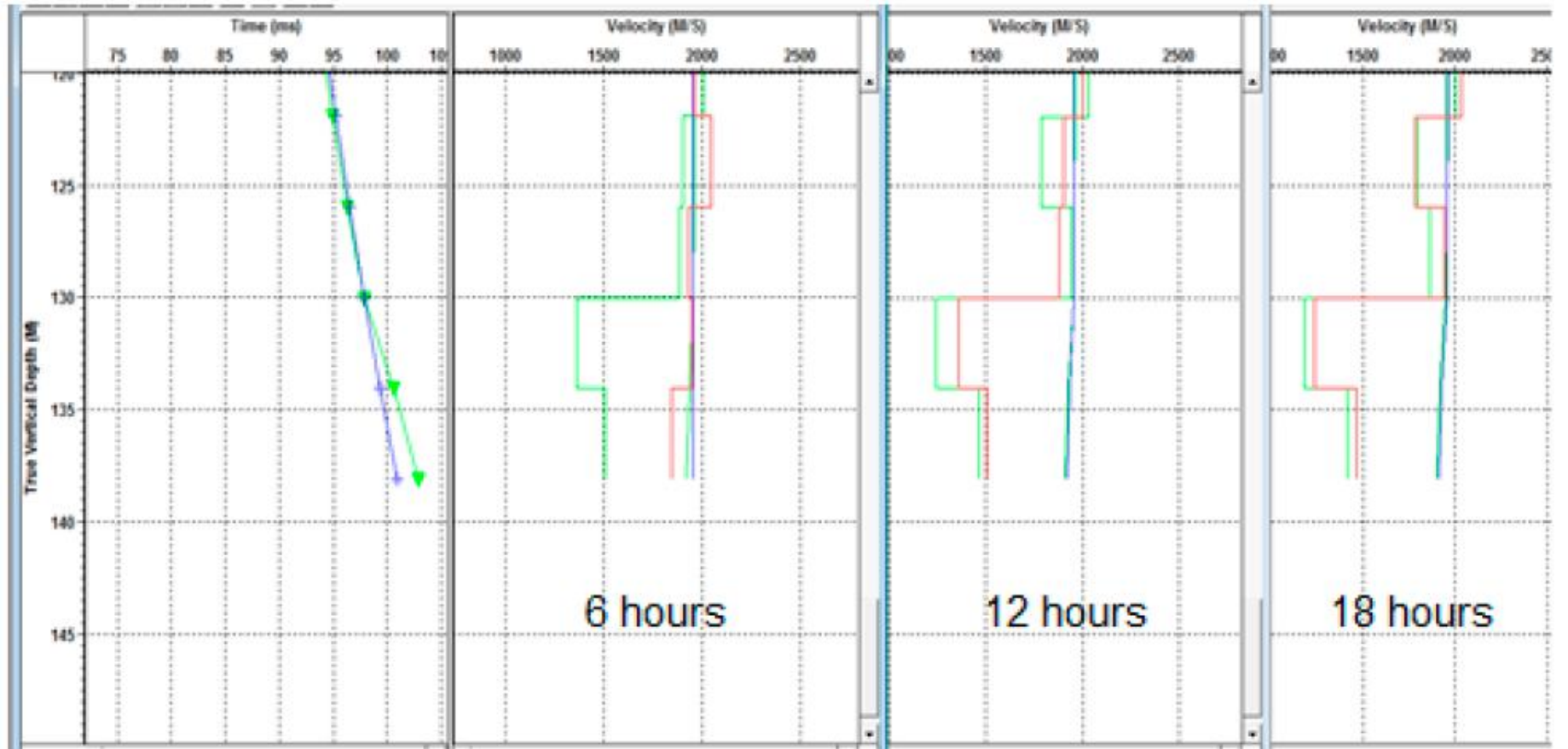
Figure 6. 1) Arrival times before injection (blue) and after 6h (green); 2) interval velocity before injection (red) and after 6h (green); 3) interval velocity after 6h injection (red) and after 12h injection (red); 4) interval velocity after 12h injection (red) and after 18h injection (red).
