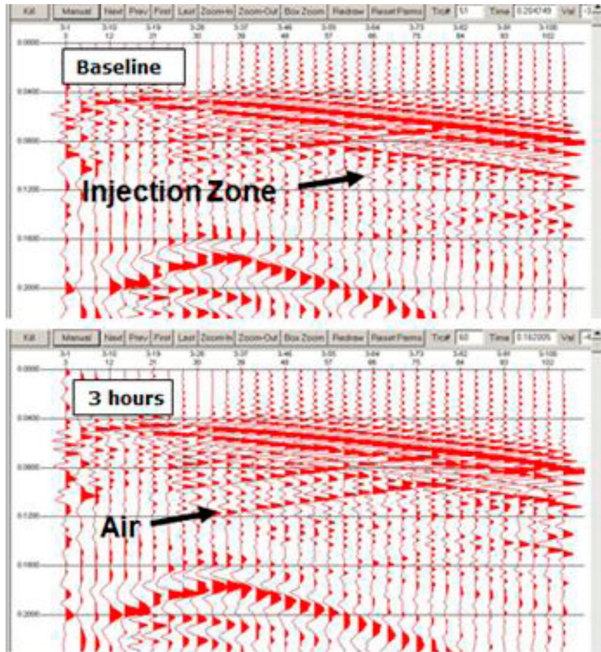
Figure 3. Single shot recordings before (top) and after three hours of air injection (bottom).
