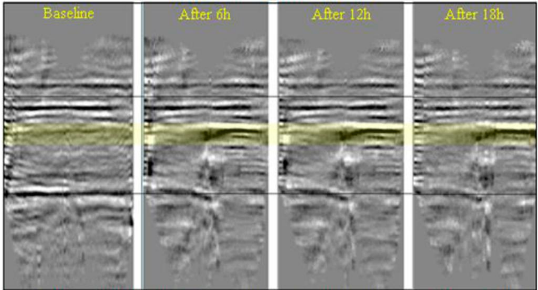
Figure 5. Extracted north/south line showing the amplitude changes with time as the air injection is performed.
