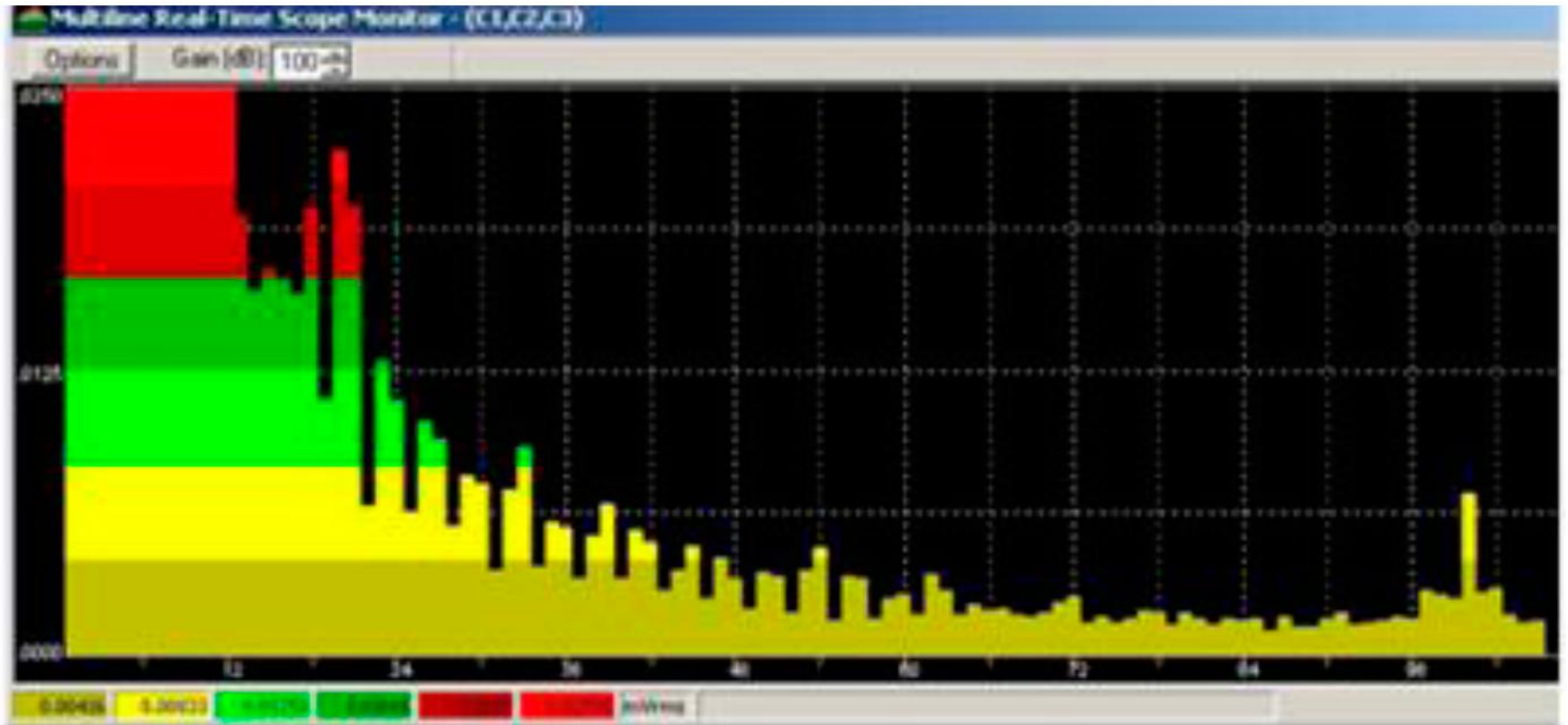
Figure 4. Screen capture of the tool noise levels during the air injection. The injection zone is on the right hand side of the image. The increase noise level from the air can be seen over the bottom tools.
