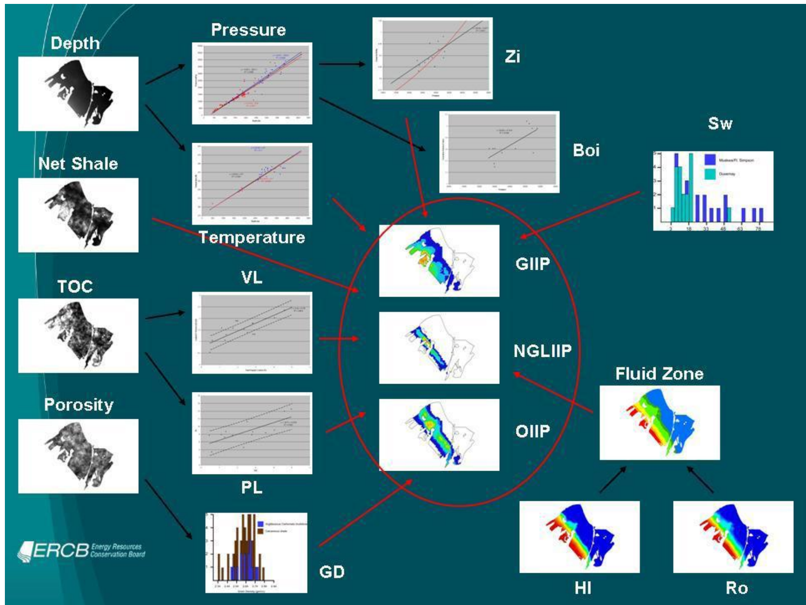
Figure 1. Simplified schematic view of the resource estimation workflow.
