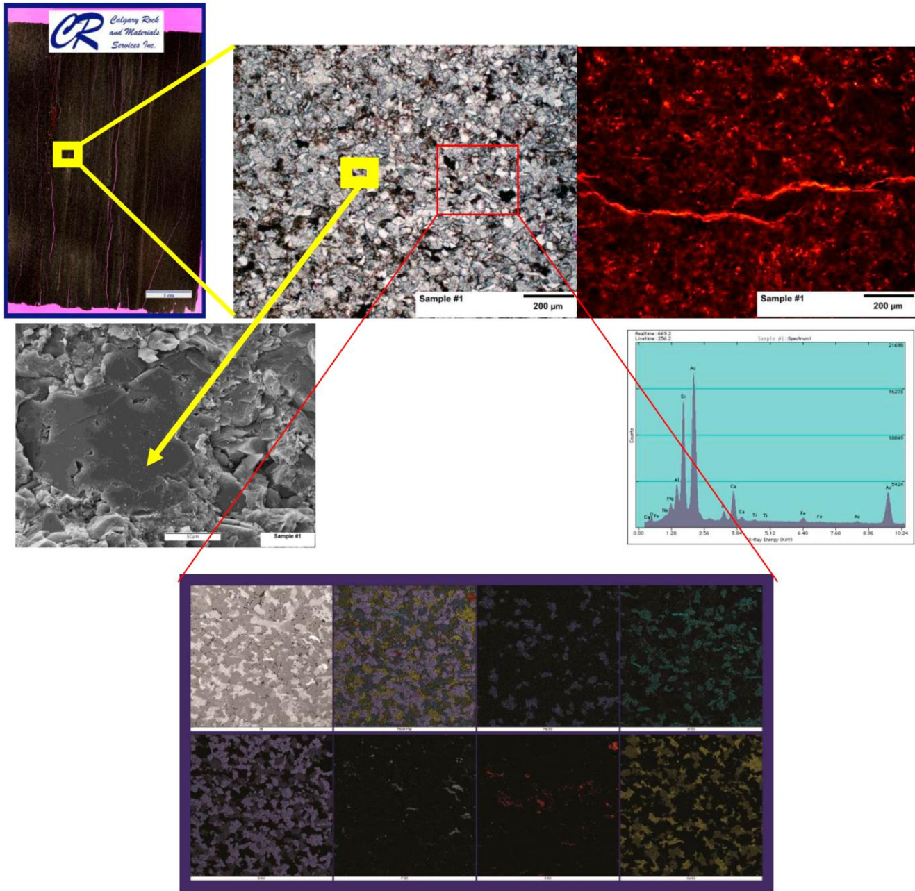
Figure 1. The integrated approach of thin section microscopy, SEM with EDS analysis, and elemental mapping.
