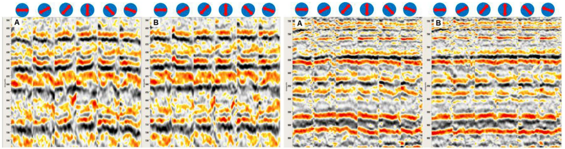
Figure 5. Comparison of two different CIG locations for six azimuths extracted from the study area. A) The gathers from the final TTI migration. Inconsistency of the residual moveout is observed through different azimuths. B) The gathers from the orthorhombic migration. Gather flatness is improved among all azimuths. Azimuths are from 0^{\circ} to 150^{\circ} with an interval of 30^{\circ} .
