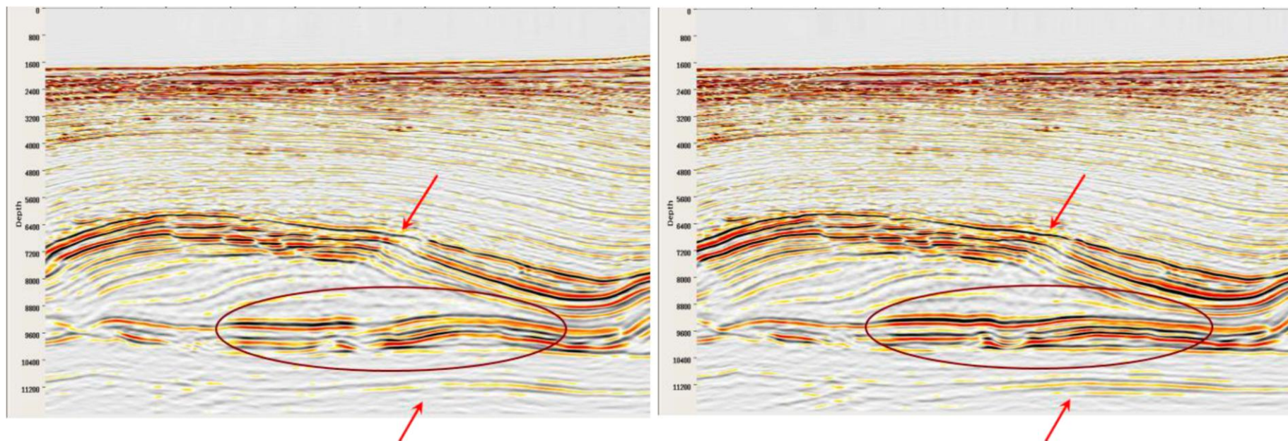
Figure 4. The stacking images for the study area. On the left is the stacking image from the TTI final migration. On the right is the one from the orthorhombic migration.
