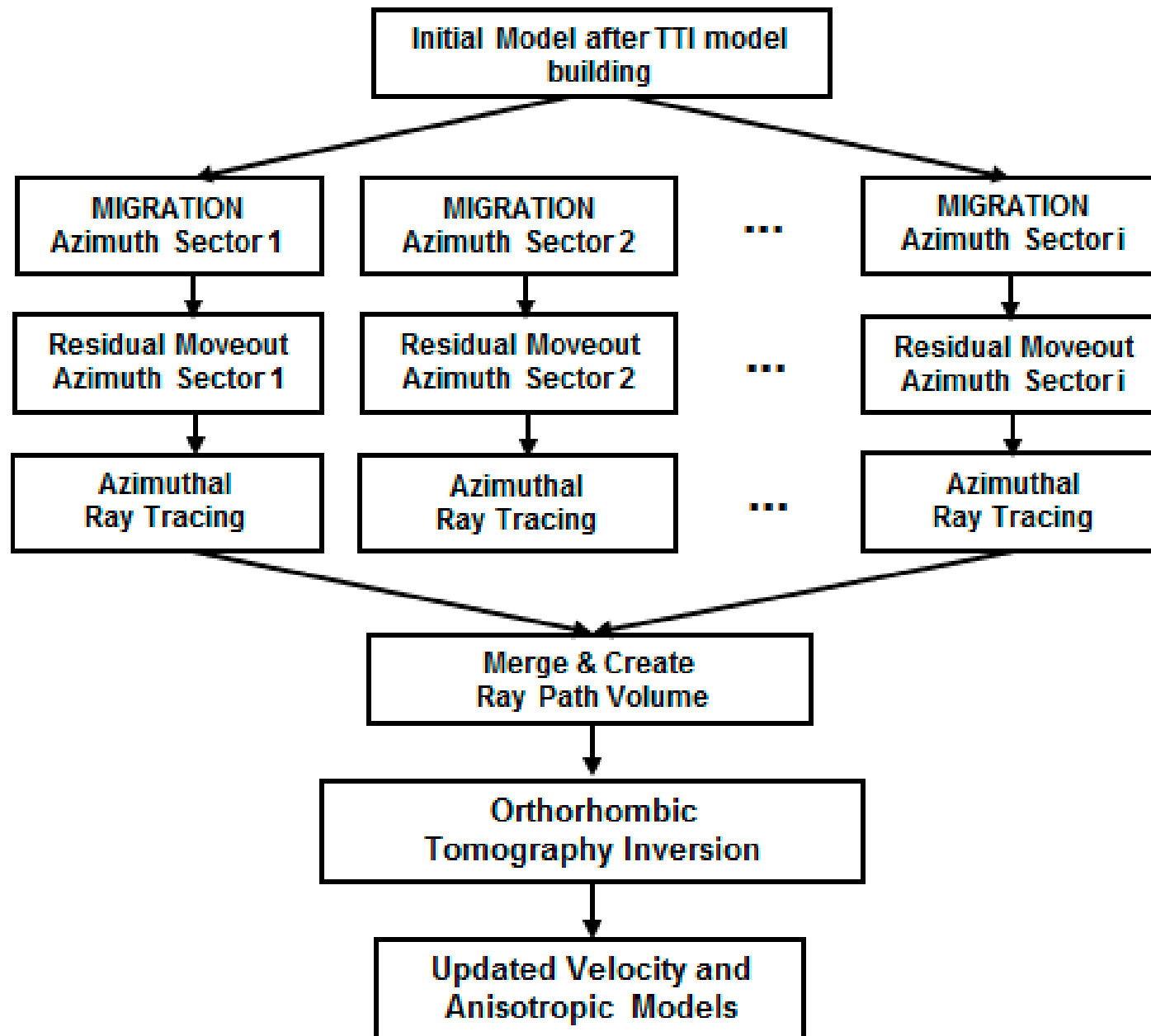
Figure 1. The workflow for orthorhombic model building.
