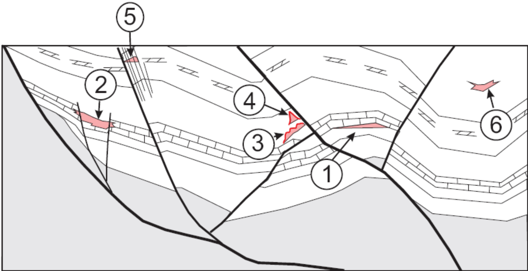
Figure 3. Schematic cross-section of the Silurian-Devonian Gaspé Belt. The 6 conventional plays are presented. Only the Lower Devonian sandstone (#6) was quantitatively assessed. See Lavoie et al (2009) for discussion for all plays.
