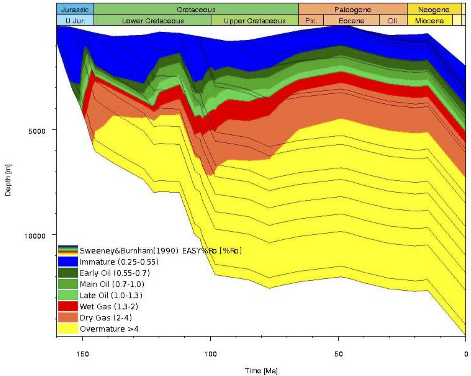
Figure 2: Maturity results of a 1D model, showing Oil and Gas window depth range.
