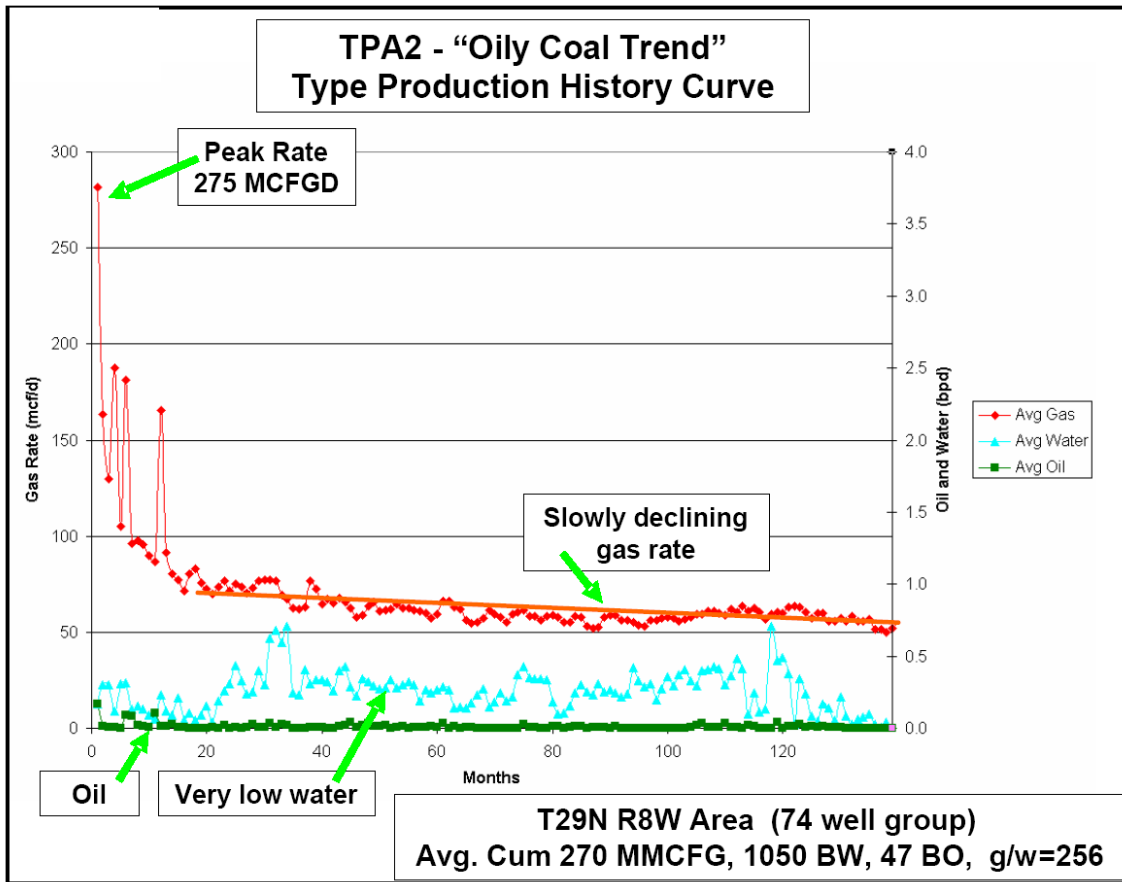
Figure 4. TPA2 - "Oily Coal Trend": Type production history curve.
