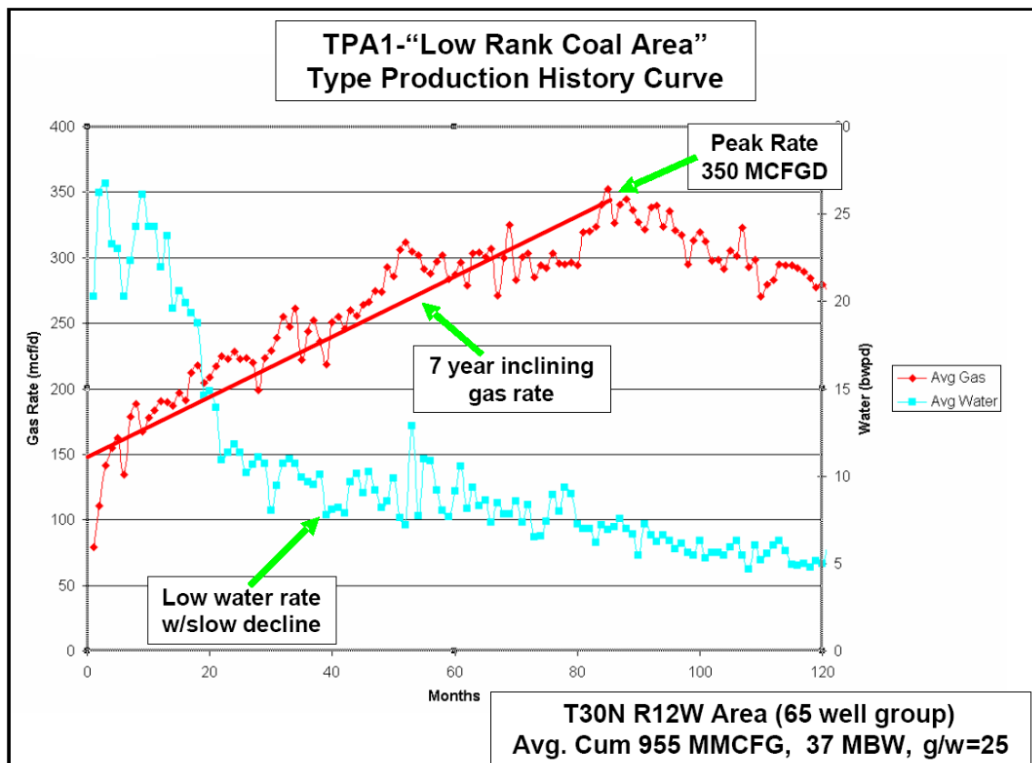
Figure 3. TPA1-"Low Rank Coal Area": Type production history curve.
