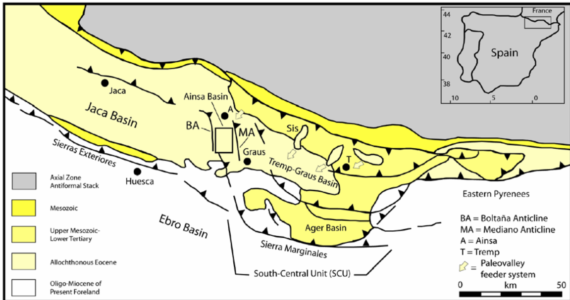
Figure 1. Main structural elements in the southern Pyrenean foreland basin. The area of Figure 2 is indicated by the rectangle. Modified from Bentham et al. (1992).
