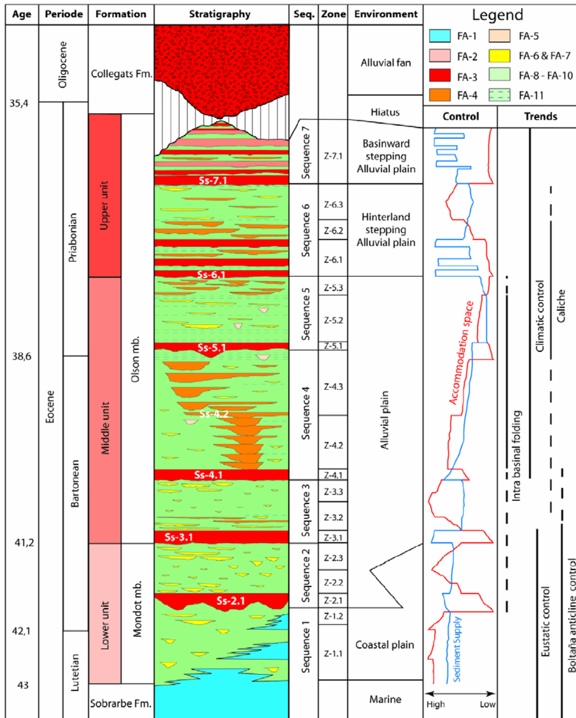
Figure 4. Summary of the sequence stratigraphic interpretation of the Escanilla Formation. The Formation is divided into seven sequences. The main controls are intra-basinal folding in interplay with climatic changes. The climate is controlling the drainage, and thus the sediment input (ages from Bentham et al., 1992).
