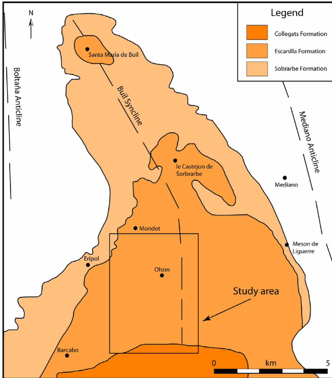
Figure 2. Geologic map of the southern part of the Ainsa Basin. Rectangle indicates the study area. The Boltaña Anticline is slightly projected from the west. Modified from Bentham et al.(1992) and Dreyer et al. (1999).
