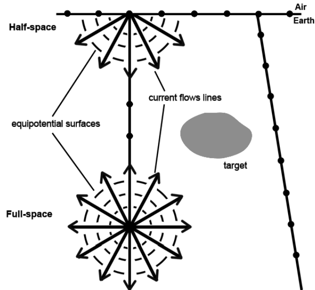
Figure 1. Schematic plot of surface and borehole electrode layout for either imaging or monitoring. Black solid circles represent surface and borehole electrodes.
