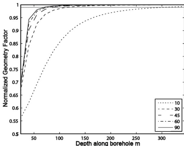
Figure 3. Geometry factors along boreholes dipping at various angles (in degrees) normalized by full-space cases. The horizontal dotted line is typical data noise level (1%). 0.5 corresponds to half-space case and 1.0 correspond to full-space case.
