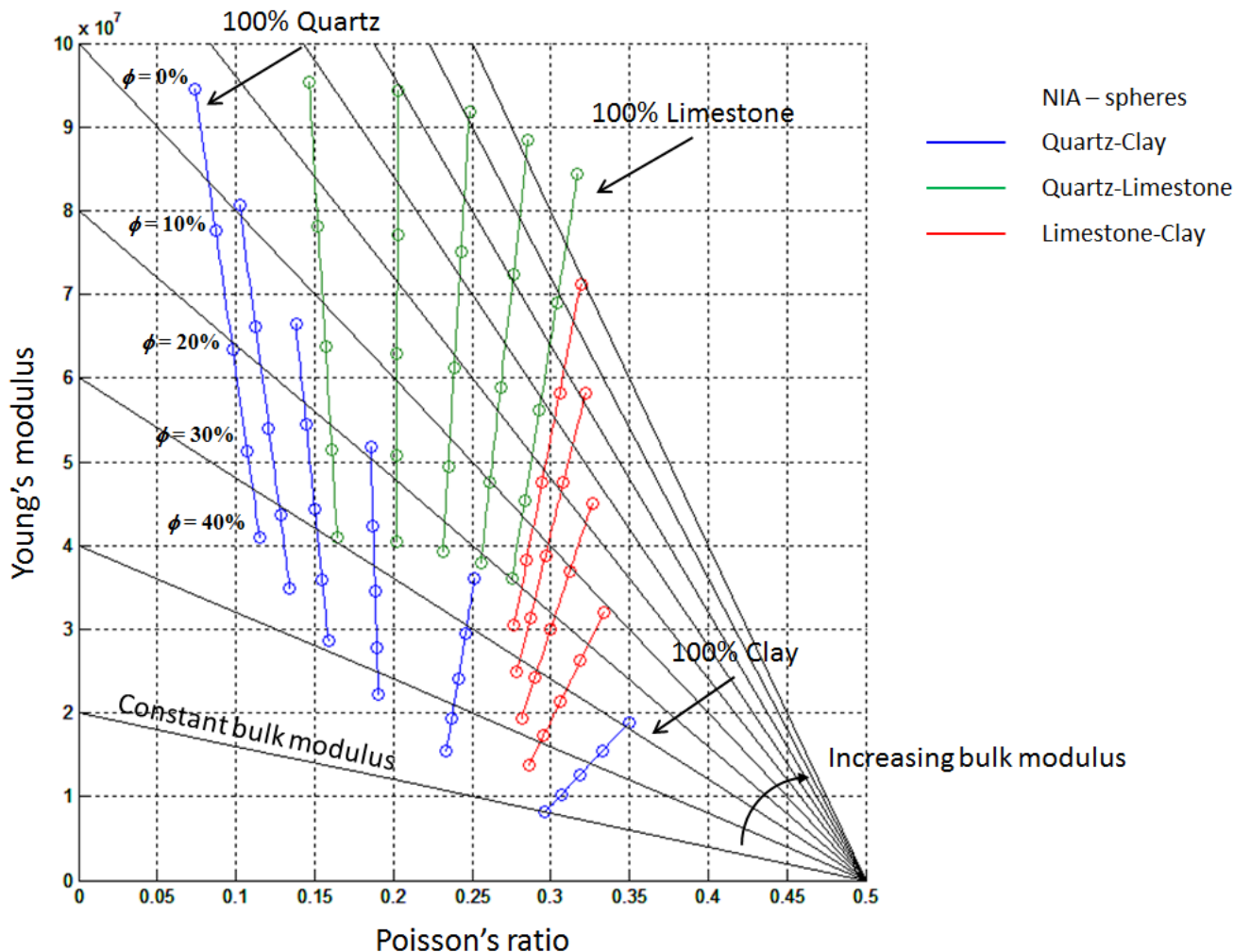
Figure 1: Rock physics trends for varying mineralogy and porosity.
