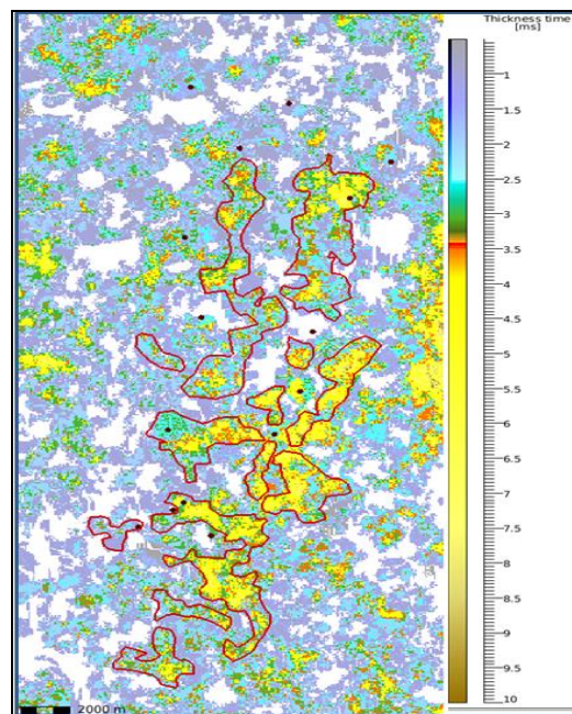
Figure 6: Sandstone time thickness map with prospective areas
