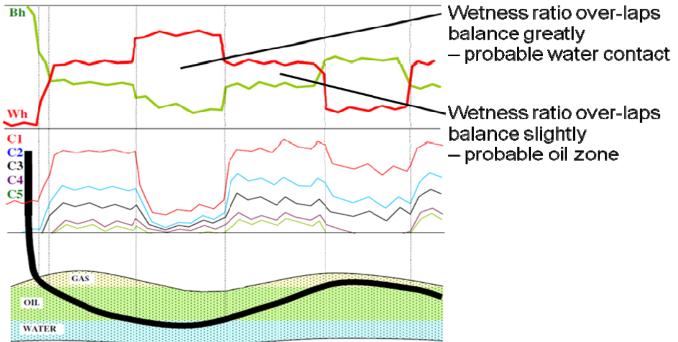
Figure 2: Using Wetness and Balance ratios for geo-steering applications.
