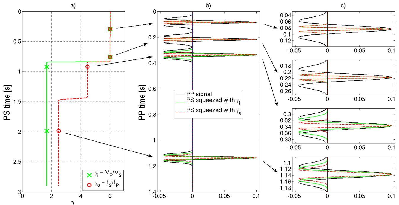
Figure 2: (a) Interval and average V_p/V_s values in PS for the same model as in Figure 1, but with values interpolated between event locations in such a way that V_p/V_s values are approximately constant in a region around each event. The PS times of four reflections are indicated by symbols. (b) A PP trace (black line), a PS trace compressed to PP time by a method that uses interval V_p/V_s , \gamma_i (green line), and a PS trace compressed to PP time by a method that uses locally constant average V_p/V_s , \gamma_{0c} (red line). (c) Close-ups of each of the four events in (b).
