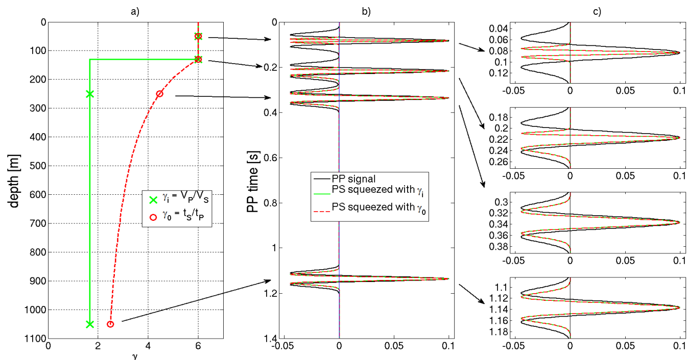
Figure 1: (a) Interval and average V_p/V_s values in depth for a simple model. The locations of four reflectors are indicated by symbols. (b) A PP trace (black line), a PS trace compressed to PP time by a method that uses interval V_p/V_s , \gamma_i (green line), and a PS trace compressed to PP time by a method that uses average V_p/V_s , \gamma_0 (dashed red line). (c) Close-ups of each of the four events in (b).
