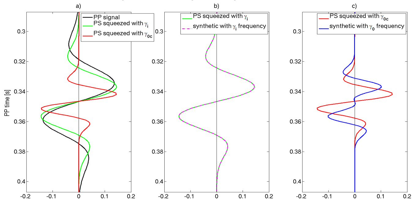
Figure 3: a) This panel is similar to the third event in Figure 2c, but the single event has been replaced by a pair of tuned events of opposite sign, located at 0.336 s and 0.356 s. b) The green line from Part a displayed together with a convolution of the reflectivity with a Ricker wavelet in which the dominant frequency has been multiplied by 2/(1+\gamma_i) . Their exact coincidence shows that reflectivity has been preserved in squeezing with \gamma_i . c) The red line from Part a displayed together with a convolution of the reflectivity with a Ricker wavelet in which the dominant
