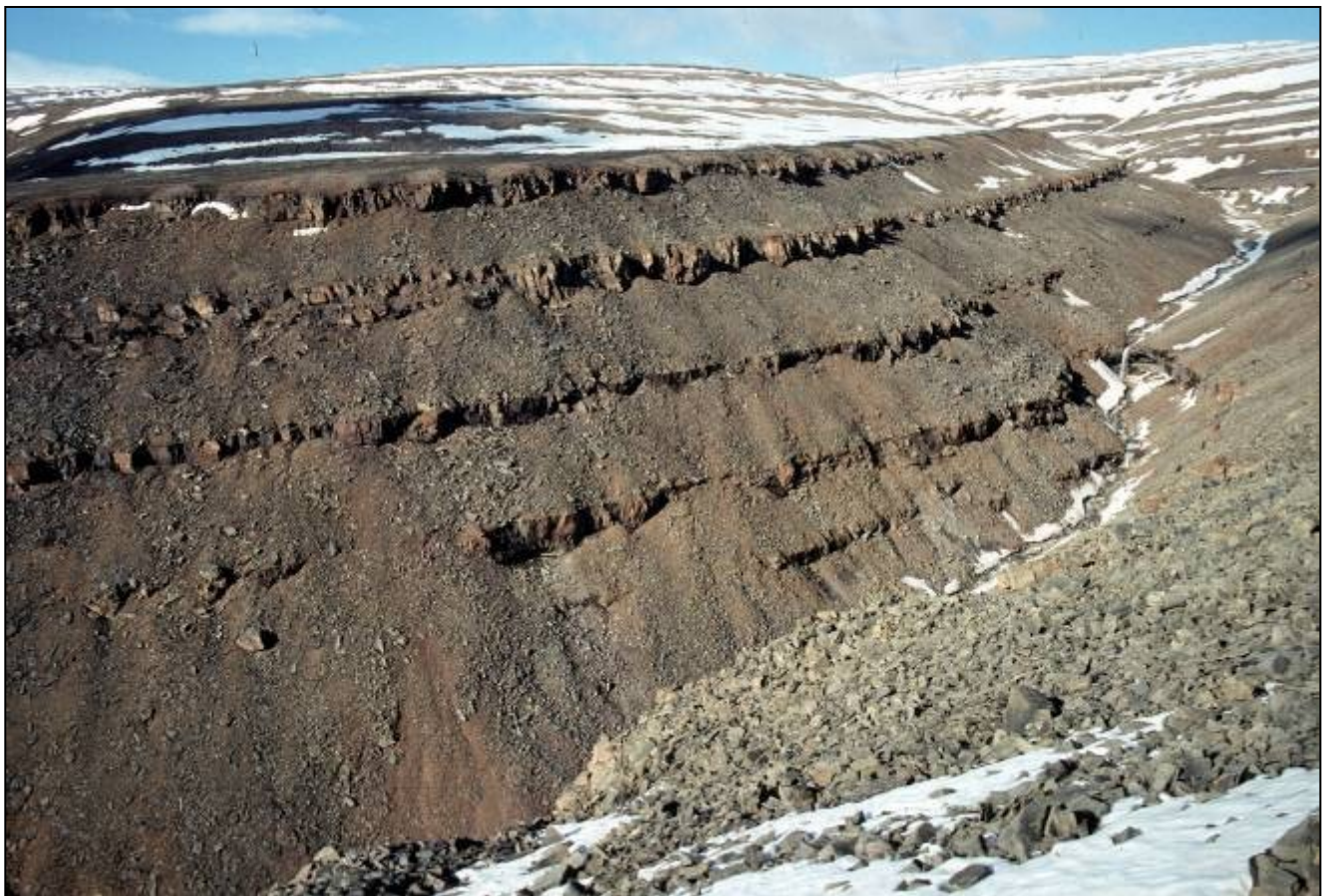
Figure 2: Sandstone-dominated red-weathering cycles, Lower Permian Canyon Fiord Formation, west Troid Fiord, southwest Ellesmere Island.
