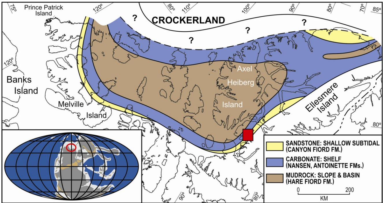
Figure 1: Study area (red square) between Blind Fiord and Troid Fiord, SW Ellesmere Island, Canadian Arctic. Insert shows location of Sverdrup Basin along NW margin of Pangaea.
