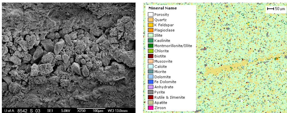
Figure 1. Left: SEM Image of a shale from the Cretaceous Colorado Group (Rokosh et al, 2008) showing a lamination of very fine sand to silt sized quartz grains. Right: QEMSCAN ® false colour image showing a similar lamination of quartz grains.
