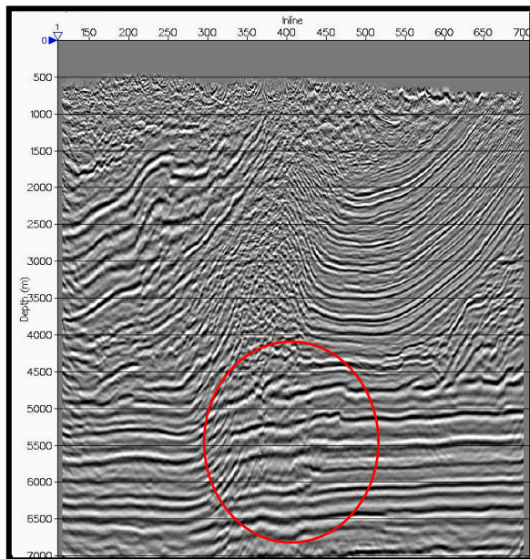
Figure 3. The final depth image shows improved reflector continuity and clearer fault.
