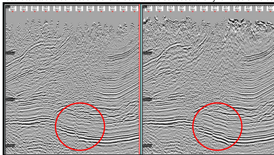
Figure 2. Structure stack of the same line as in Figure 1 shows a comparison of stacks with conventional statics calculation (left) and new de-migration statics calculation (right).
