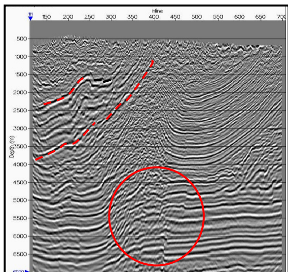
Figure 1. PSDM inline showing distortions on base carbonate layers (in red circle). The dashed lines outline the carbonate thrust sheet.
