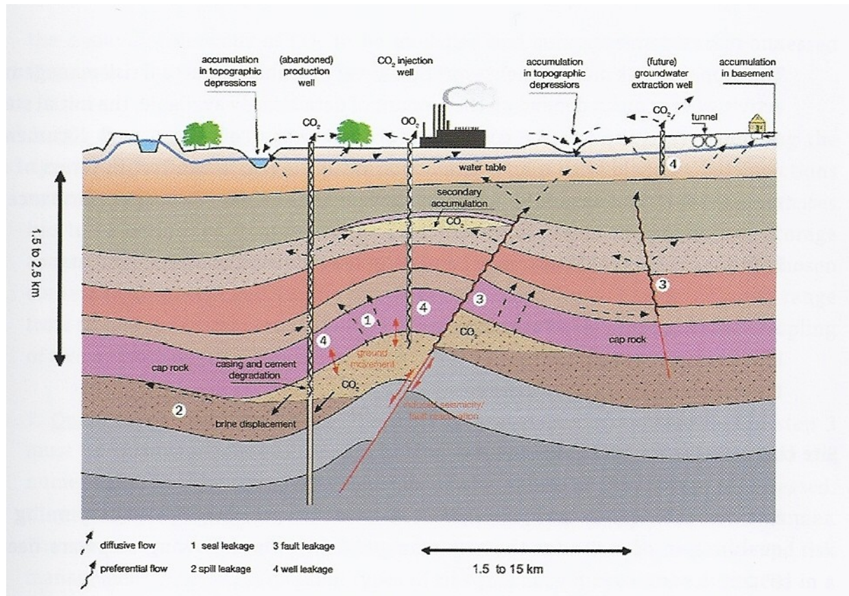
Figure 2: Main leakage paths for CO 2 to move toward the surface: 1) Seal Leakage; 2) Spill Leakage; 3) Fault leakage; 4) Well leakage. From Pagnier, 2009.
