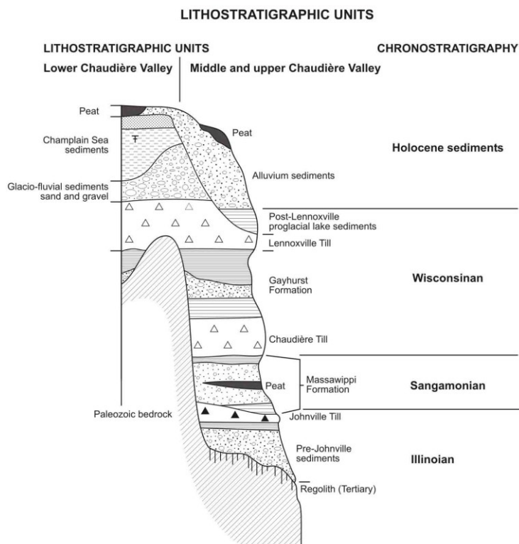
Figure 1: Quaternary lithostratigraphic framework for the Chaudière River Basin, (modified from McDonald and Shilts, 1971; and Shilts, 1981). The elevated portion of the bedrock is a schematic representation of the Notre-Dame Mountain Anticlinorium as it marks the approximate limit between the St-Lawrence Lowlands to the West and the Appalachians to the East. A simplified stratigraphic scheme is shown for the Lower Chaudière Valley.
