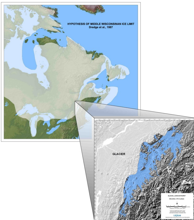
Figure 2: The maximum extent of MidWisconsinan Glacial Lake Gayhurst. As the normal drainage is from the International Border towards the St. Lawrence River, any ice expansion across the St- Lawrence Valley, and into the Appalachians would have created ice-dammed lakes, during each glacial advance and northward retreat.
