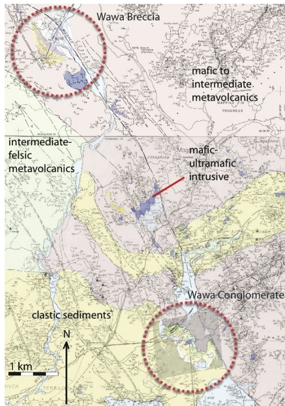
Fig. 1: Geologic map and locations of the diamondiferous suites of Wawa, Northern Ontario (Canada).
