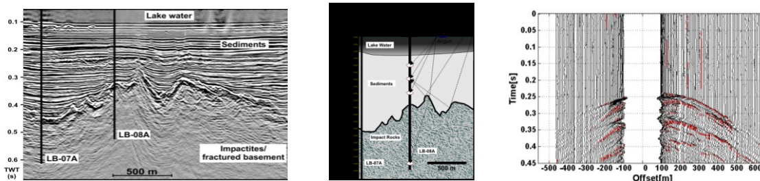
Figure 1: a) Depth (two-way travel time: TWT) section acquired via multichannel surface seismic Survey (Scholz et al., 2002). Borehole LB-08A was drilled through the central uplift whereas LB-07A was drilled at the outer rim of the uplift. Note absence of reflections in the hard rock (fractured basement) environment; b) Cartoon of Offset VSP acquisition geometry; c) Scaled amplitude plots of the offset VSP data for the receiver at 450m depth. Gaps in the data represent locations with no information.
