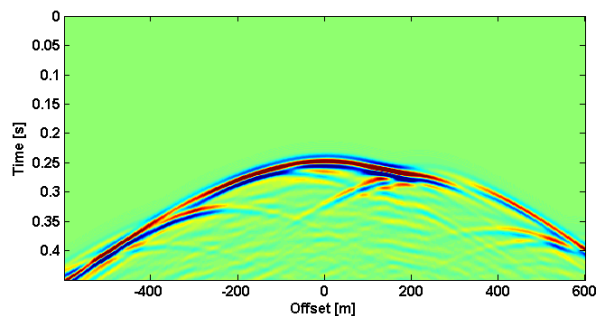
Figure 2: Vertical component plot of the recorded wavefields (synthetic) at the receiver locations (Trace interval 2.4m). Note the asymmetry of the recorded wavefield about the borehole location (0m offset).
