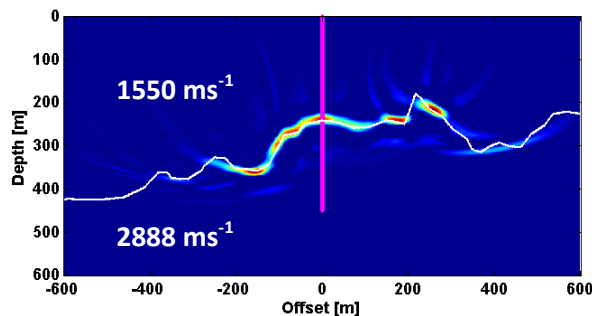
Figure 3: Reconstructed sediment-breccia contact image using the migration method. The superimposed white line represents the true model contact. The P-wave velocities are for the soft sediments and the breccia unit respectively.
