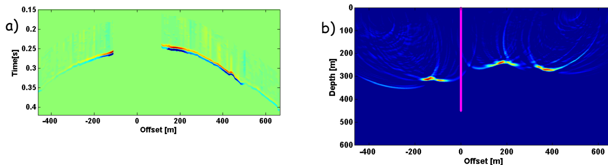
Figure 4: a) Preprocessed data from R-450 (muting and trace interpolation). Traces for small absolute offsets (<100m) were padded with zeros; b) Reconstructed sediment-breccia contact image from R450 using the migration method.
