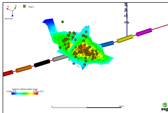
Figure 2: Seismic deformation analysis for a single hydraulic fracture treatment stage. Colored contours illustrate that higher levels of deformation occur directly around the treatment zone, indicating good communication with the treatment zone.
