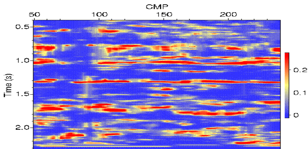
Figure 3: Attenuation section.
