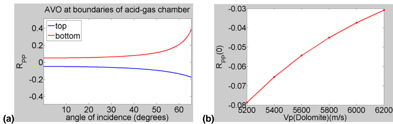
Figure 2: (a) Reflection coefficient curves defining R_{PP}(\theta) at the top and bottom of an acid gas layer. The rock matrix is assumed to be constant across the interfaces, with brine saturation above and below the reservoir. (b) The effect of reservoir rock V_P on vertical reflectivity [ R_{PP}(0) ] at the top of the injection chamber, given the same assumptions as in Figure 1.
