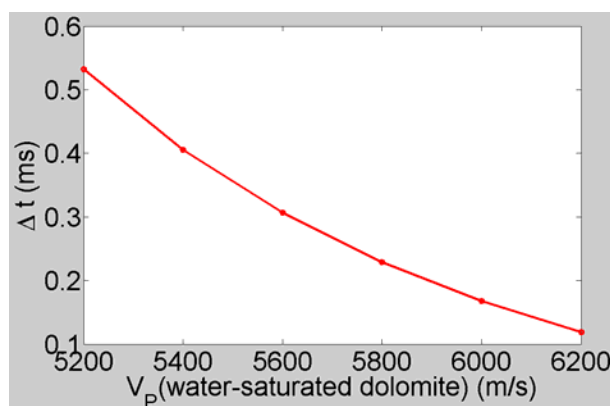
Figure 1: The effect of reservoir rock V_P on two-way traveltimes differences resulting from fluid substitution.
