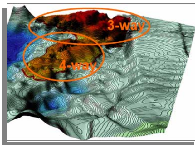
Figure 2: The Ernest Prospect with a 4-way closure and a 3-way closure (Rockhopper, 2006)
