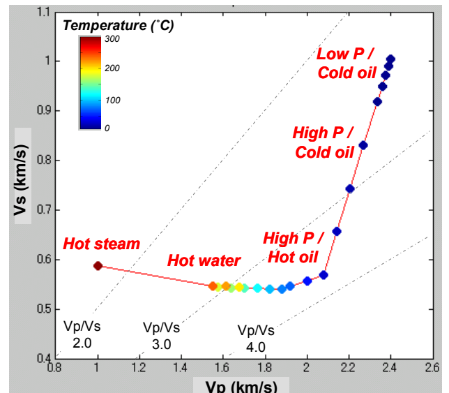
Figure 3: Sequential rock physics model for bitumen reservoir and cross plot between P- and S-wave velocities during steam injection based on the model
