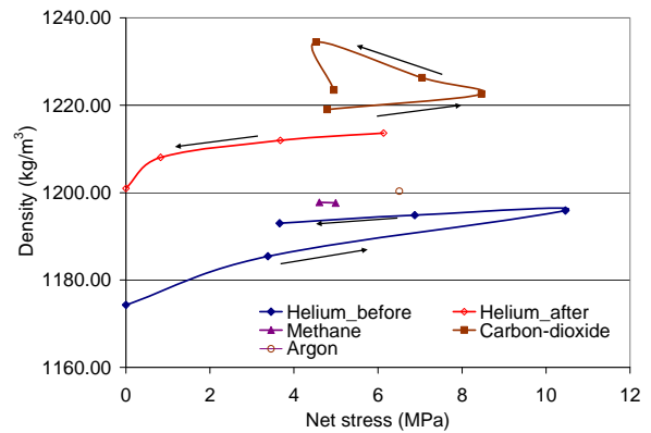
Figure 4: Coal average bulk density change
