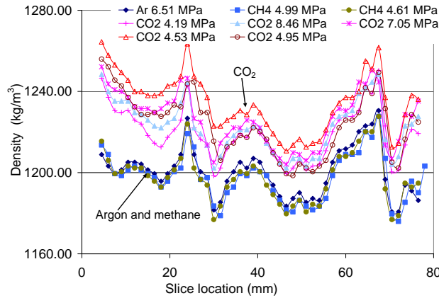
Figure 3: Density log with CO 2 at different net overburden pressure
