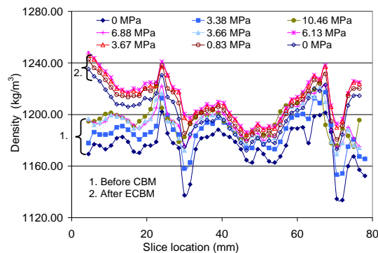
Figure 2: Density log for helium flow at different net overburden pressure
