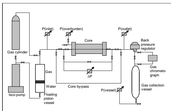
Figure 1: Schematic of the core-flood rig
