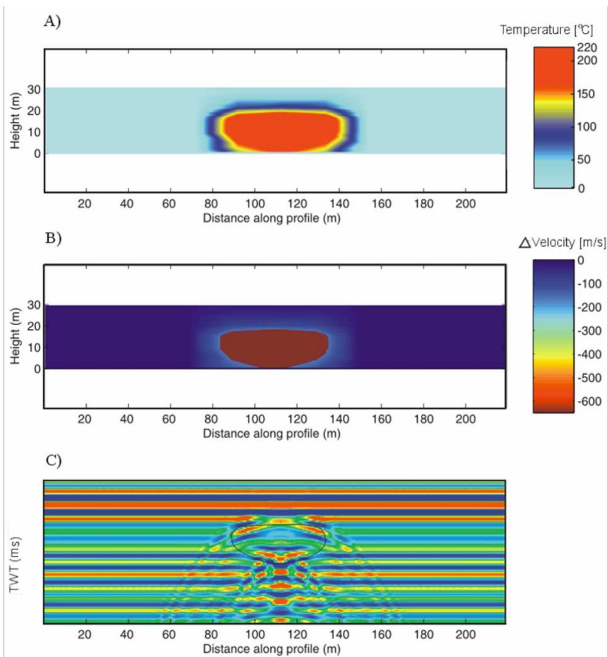
Figure 3: A) Hypothetical temperature profile of a typical steam chamber in Athabasca reservoir B) Computed P-wave velocity anomaly result from rock physics and fluid substitution analysis. C) Un-migrated synthetic seismic profile generated using an acoustic finite difference algorithm. The steam anomaly in B) is superimposed on the background reflectivity determined by closely spaced well logs at the UTF. The offset range used in this stacked section is 48 -142m.
