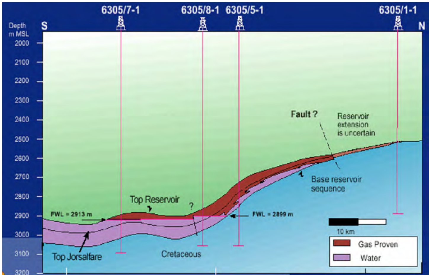
Figure 4 Simplified section through reservoir
