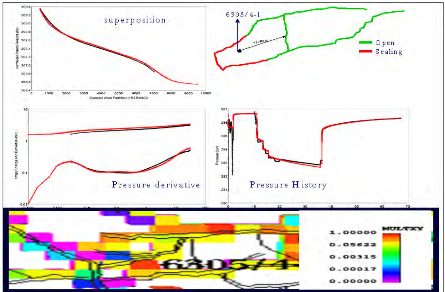
Figure 5 Test Result well 6305/4-1
