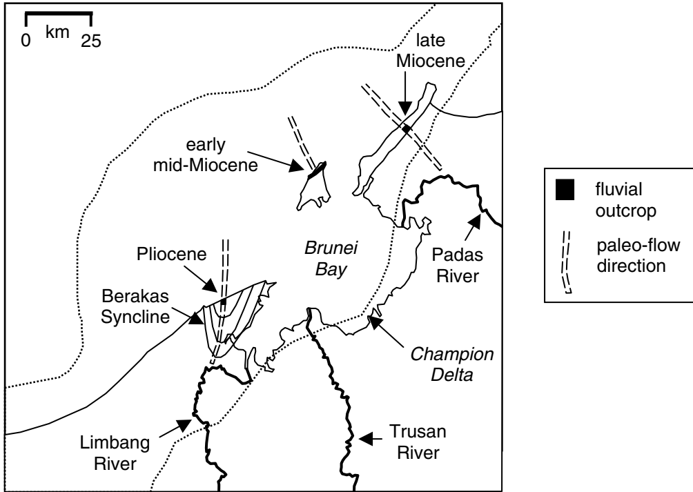
Figure 2. Fluvial outcrops, major rivers and palaeo-flow directions within the Brunei Bay drainage basin.
