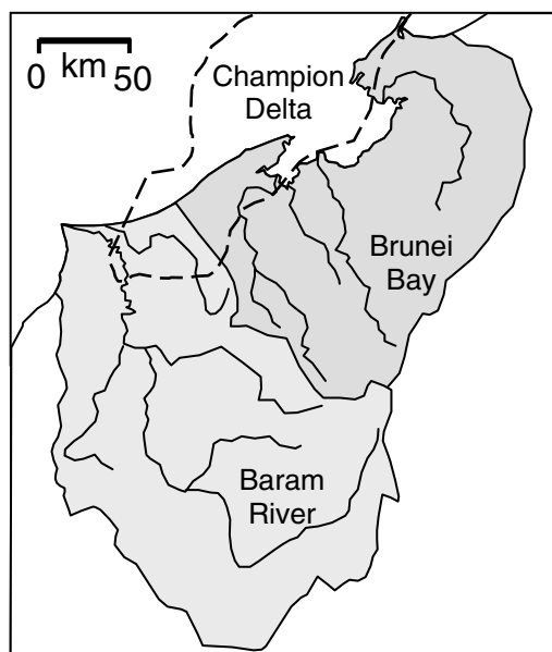
Figure 1. The Baram River and Brunei Bay drainage basins and the location of the Champion Delta (after Sandal, 1996).
