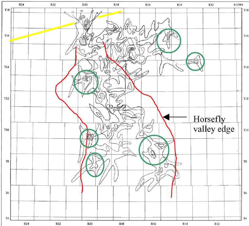
Figure 2: Isopach map (black lines) showing the palaeomorphology of the BAT incised-valley fills. Note the presence of thicker deposits at the junctions of tributaries (green circles). The yellow line indicates the approximate location of the Vulcan structure. Isopach interval = 10 m.
