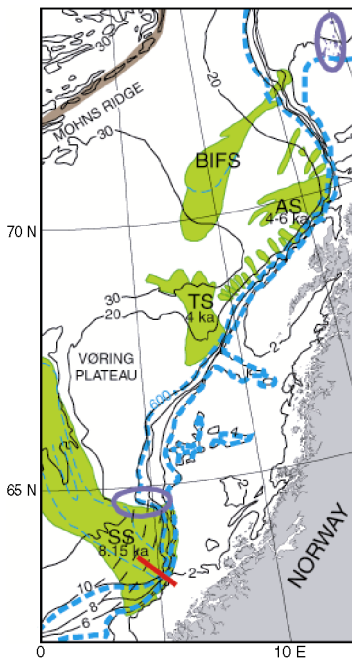
Figure 1. Norwegian continental margin, showing relatively recent giant underwater landslides in green: SS, Storegga slide; TS, Traenadjupet slide; AS, Andoeya slide; and BIFS, Bear Island Fan slide. Gas hydrate stability models shown in Figures 2 and 3 were computed along red line. Black contours show water depths in 100s of meters; thickness of modern methane hydrate stability zone, in meters, shown by dashed blue contours (600m and 0m). Blue ovals and patches show areas where seismic surveying has detected hydrates.
