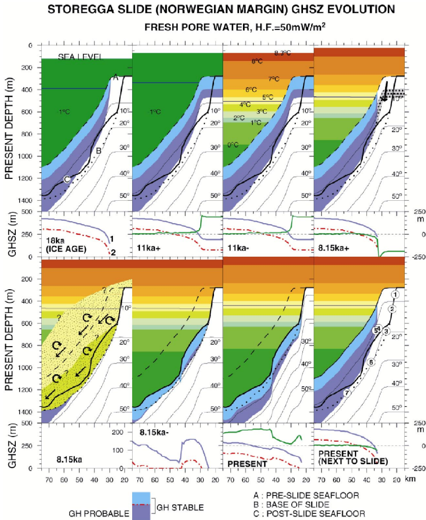
Figure 2. Computed changes in gas hydrate stability zone (GHSZ) over time from last glacial maximum (18,000 years ago, or 18ka) to ocean warming at 11ka, Storegga landslide at 8.15ka, and to present conditions in slide area and on adjacent, not (yet) failed seafloor. 11ka+ means just prior to 11,000 years ago, etc. Stippled zone in 8.15ka+ profile shows area of hydrates dissociated from previous profile (11ka-). Top of each profile is modern sea level. The sub-seafloor GHSZ is shown in blue, with the upper 115m (light blue) probably lacking hydrate. Horizontal blue line is upper limit of GHSZ in ocean. Dashed line (A) shows the restored, pre-slide seafloor, heavy line (B) is the present seafloor, and dotted line (B) is the failure surface (base of slide). Conditions during the actual slide(8.15ka) are schematic only. Small numbers show points whose trajectories in (P, T) space are shown in Figure 3.
