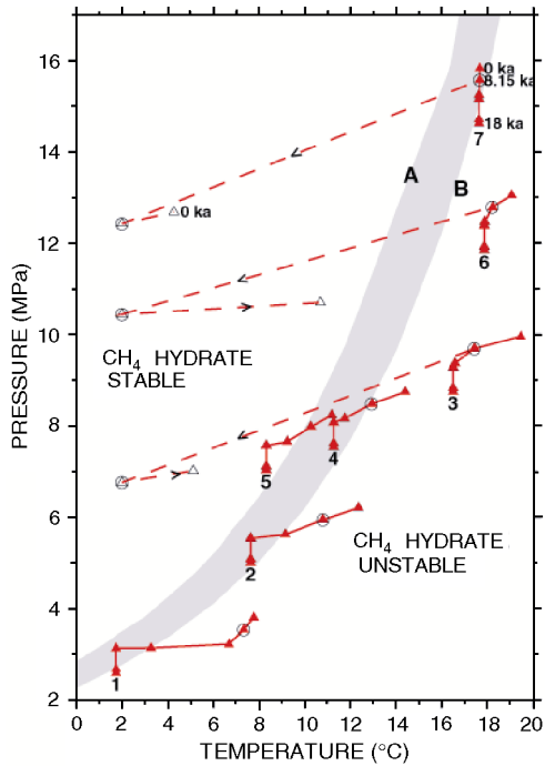
Figure 3. Trajectories (from last Ice Age at 18ka, to the present) of seven sub-seafloor points (See Fig. 2 for locations) in Temperature and Pressure space, in relation to boundary of methane hydrate stability. Circled points correspond to 8.15ka, time of Storegga slide. Trajectory branches for points within the slide area and covered by slide debris are shown dashed. Because the phase boundary depends on pore water salinity and admixed higher hydrocarbons, it is shown here as a band. The left edge (A) reflects pore water with the salinity of seawater, while the right edge (B) reflects fresh water with 2% ethane.
