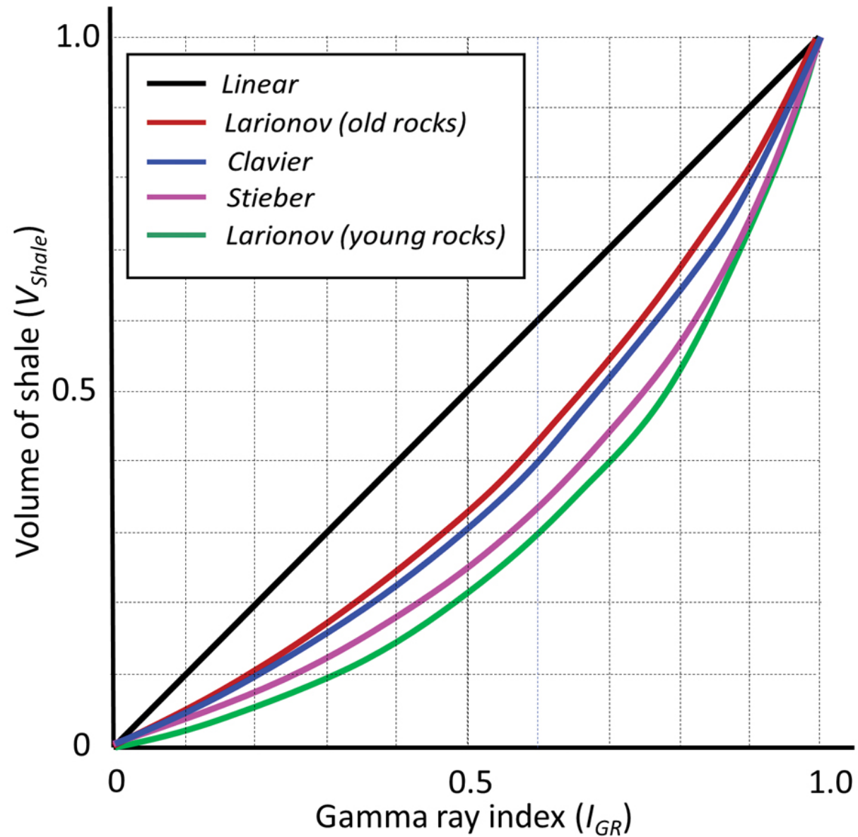
Figure 1. A crossplot showing the variation of the volume of shale as a function of gamma-ray index. The solid black line is the linearly scaled data, the colored lines represent the different corrections applied to the data as shown in the legend.
