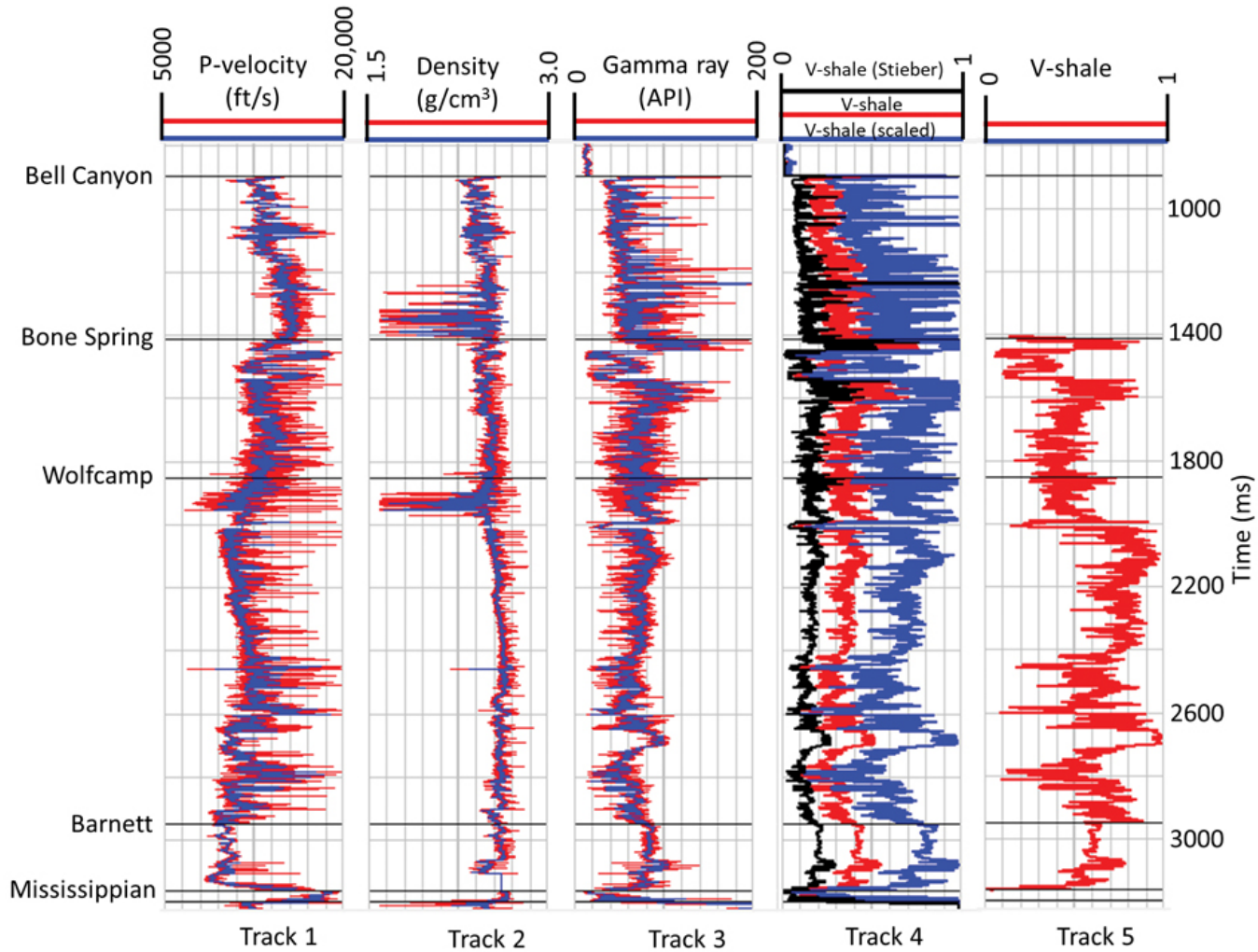
Figure 2. The sonic, density and gamma-ray curves from a well in the Delaware Basin in west Texas and New Mexico in the United States are shown in tracks 1, 2 and 3. The red curves show the input curves as such and the blue curves are their smoothed versions, which were used in the computations. The volume of shale curves corrected using scaling and Stieber corrections are shown in track 4. The volume of shale was also computed by a petrophysicist by first subdividing the curves into five basic zones, the prominent ones being the Bone Spring, Wolfcamp and the Barnett/Mississippian intervals. Next, the minimum and maximum values of the gamma-ray log in the respective zones were picked up. Finally, the computations of the gamma-ray index were merged into a single composite curve, shown in track 5.
