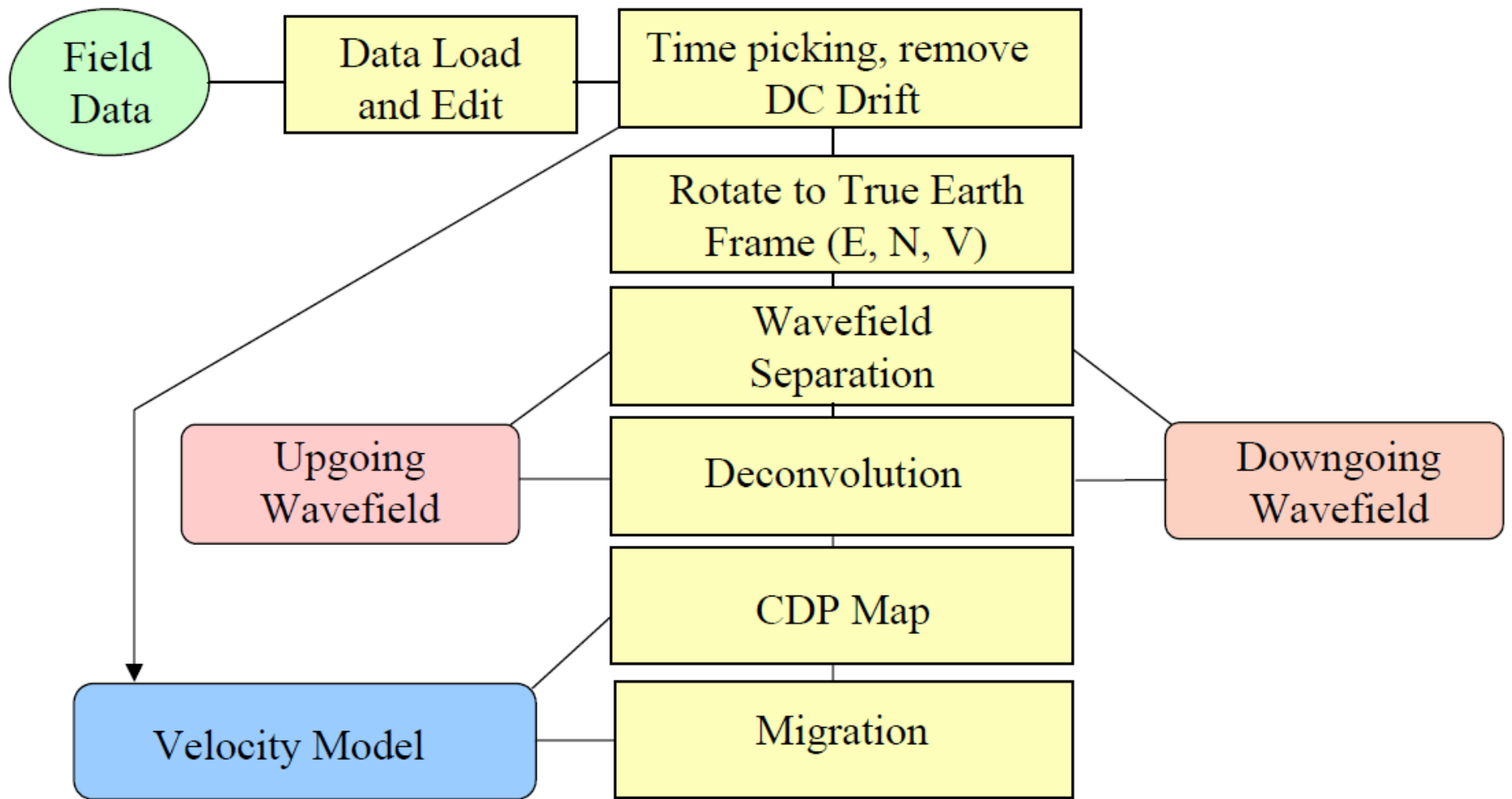
Figure 2. VSP processing flow used for the baseline and monitor surveys.
