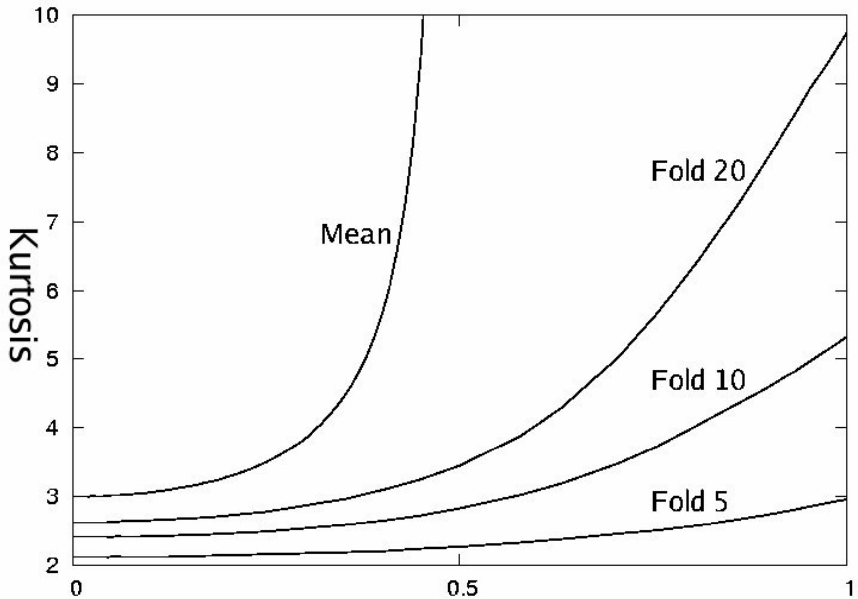
Figure 2. Kurtosis as a function of \lambda . “Mean” is the expected mean of the Kurtosis. The rest are the expected median of the kurtosis for various folds.
