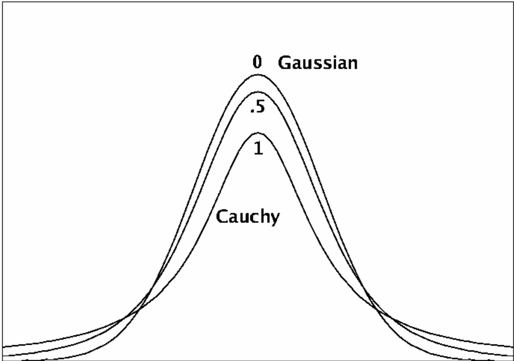
Figure 1. Student's t-distribution for \lambda = 0 (Gaussian), .5 , and 1 (Cauchy). Note that the tails get fatter as \lambda increases.
