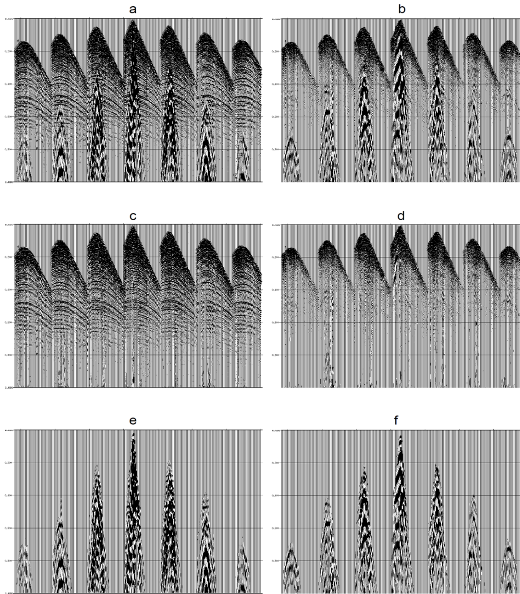
Figure 3. Results of polarization filter on a 3C 3D data: (a) raw shot records of vertical components, (b) raw shot records of radial components, (c) vertical components after polarization filter, (d) radial components after polarization filter, (e) difference of vertical components, (f) difference of radial components.
