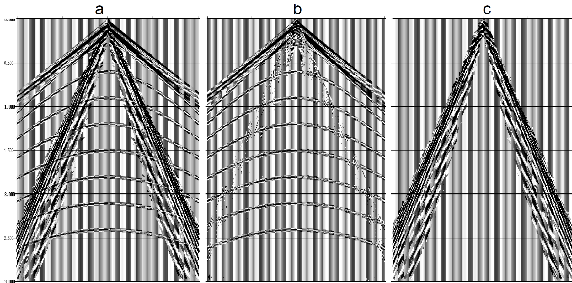
Figure 2. Ground roll attenuation on horizontal-inline components of synthetic data: (a) a shot record containing high-amplitude ground roll, (b) after polarization filter, (c) the difference.
