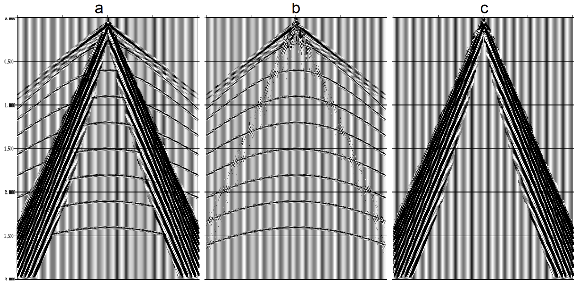
Figure 1. Ground roll attenuation on vertical components of synthetic data: (a) a shot record containing high-amplitude ground roll, (b) after polarization filter, (c) the difference.
