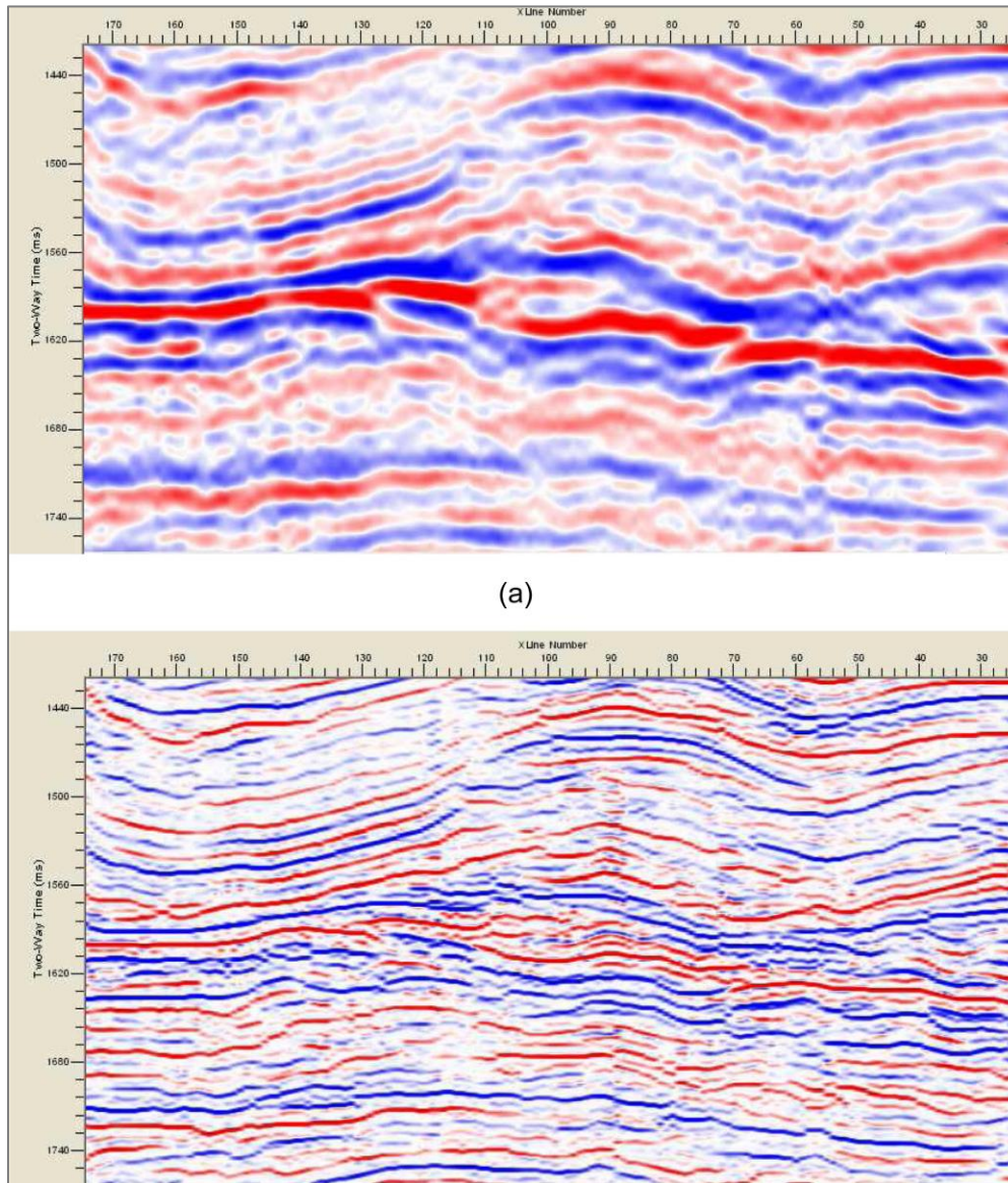
Figure 1. Shows a comparison of (a) the band-limited seismic section and (b) the equivalent derived thin-bed reflectivity section. The display contrast for the reflectivity has been enhanced purposely to bring out the resolution detail that can be seen. Data courtesy of Arcis Corporation, Calgary.
