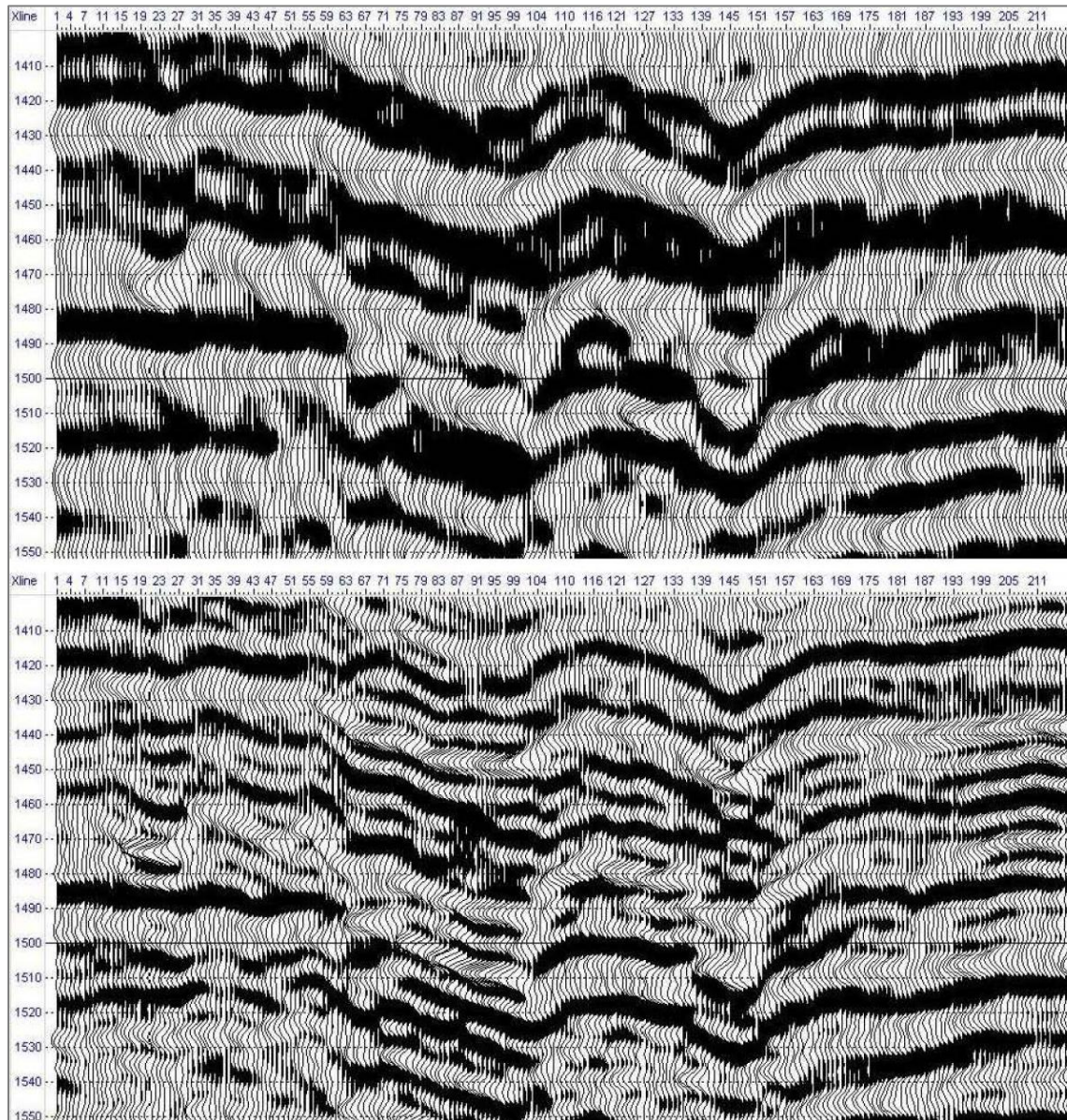
Figure 3. This figure shows a segment of a seismic section from the input seismic data and the same segment from the reflectivity volume convolved with a bandpass wavelet with a high end of 120 Hz. Notice the higher resolution that has been achieved as well as the fact that lateral changes in wavelet character can now be studied. Data courtesy of Arcis Corporation, Calgary.
