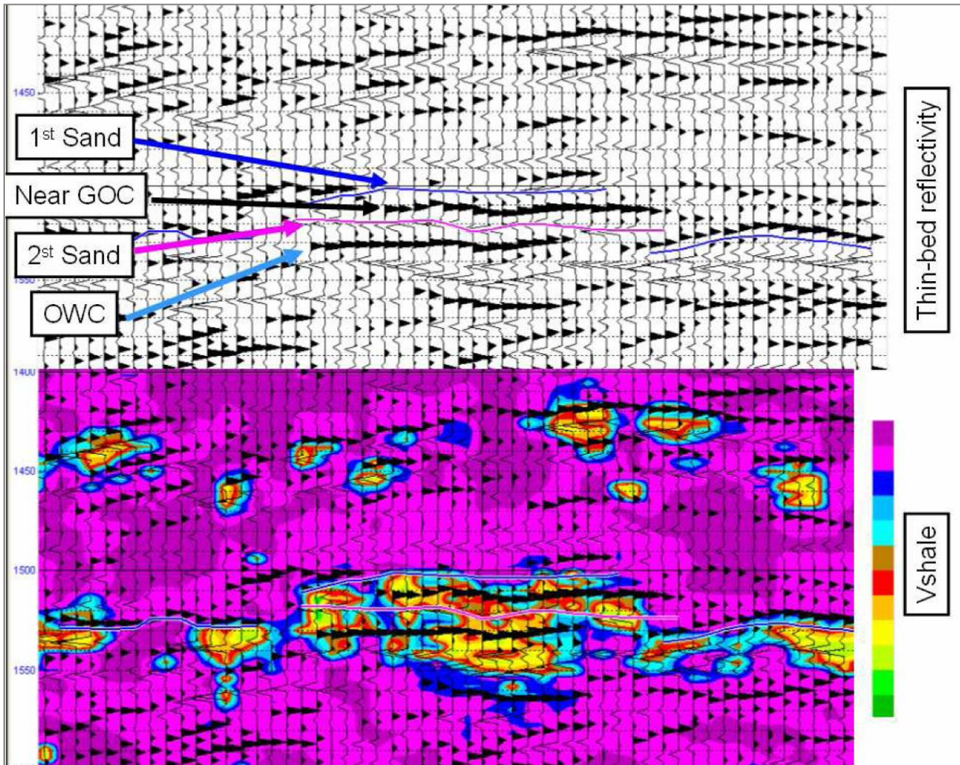
Figure 2. The thin-bed reflectivity inversion allows picking individual sand intervals (upper figure) while the neural network solution displays one sand-body only (lower figure). However, only the combined interpretation of the V_{shale} and the reflectivity volume makes the correlation from one channel to the next successful. The flat spot, which marks the OWC, can be correlated and serves as a tool to identify hydrocarbons. The seismic section is tied to several wells. Data courtesy of Oilexco, Calgary.
