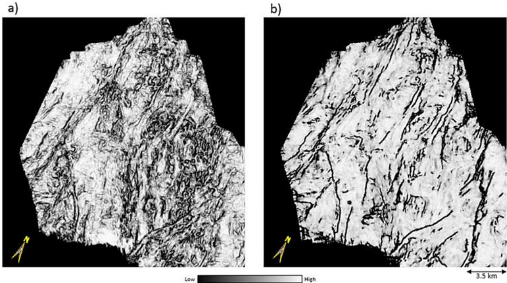
Figure 1. Stratal slices from a horizon picked close to t=1200 ms through (a) Sobel filter similarity, and (b) energy ratio coherence volumes. Although both “coherence” algorithms used the same structurally-oriented filtered data volume as input and the same 5-trace by \pm 10 ms analysis window, these two images are quite different, with the Sobel filter similarity showing more stratigraphic features and the energy ratio coherence providing sharper fault images.
