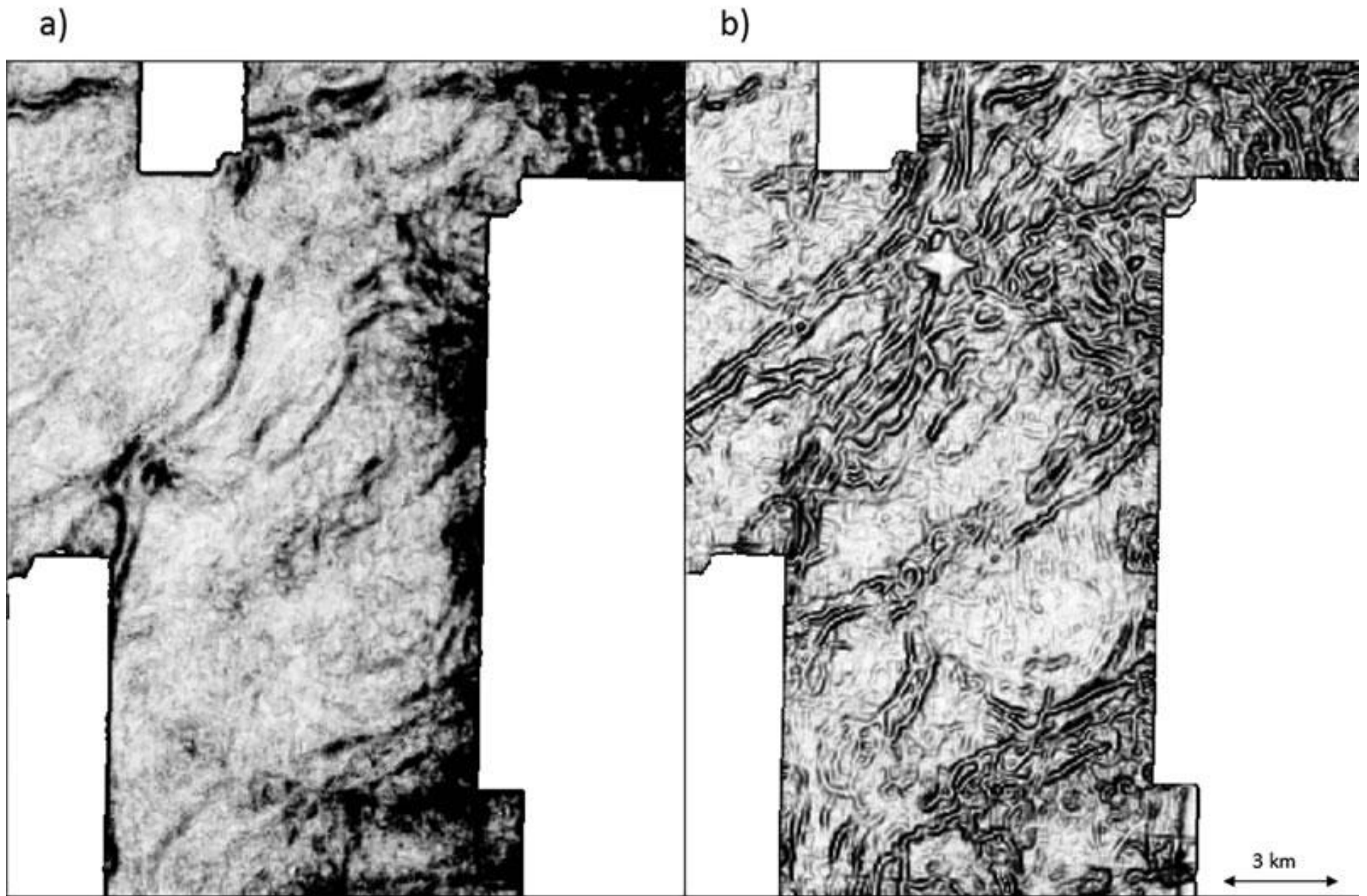
Figure 3. Time slice at t=1020 ms from (a) coherence volume computed using the energy ratio algorithm, and (b) Sobel-filter run on the coherence shown in (a). Notice the clarity with which the edges of channels seen in (a) are seen in (b).
