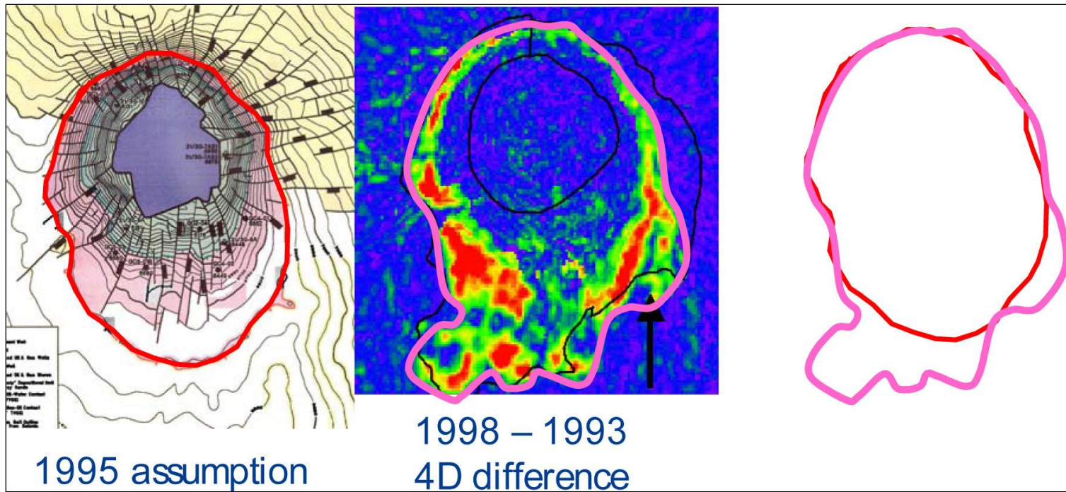
Figure 5. Oil-water contact assumptions compared before and after 4D seismic.
