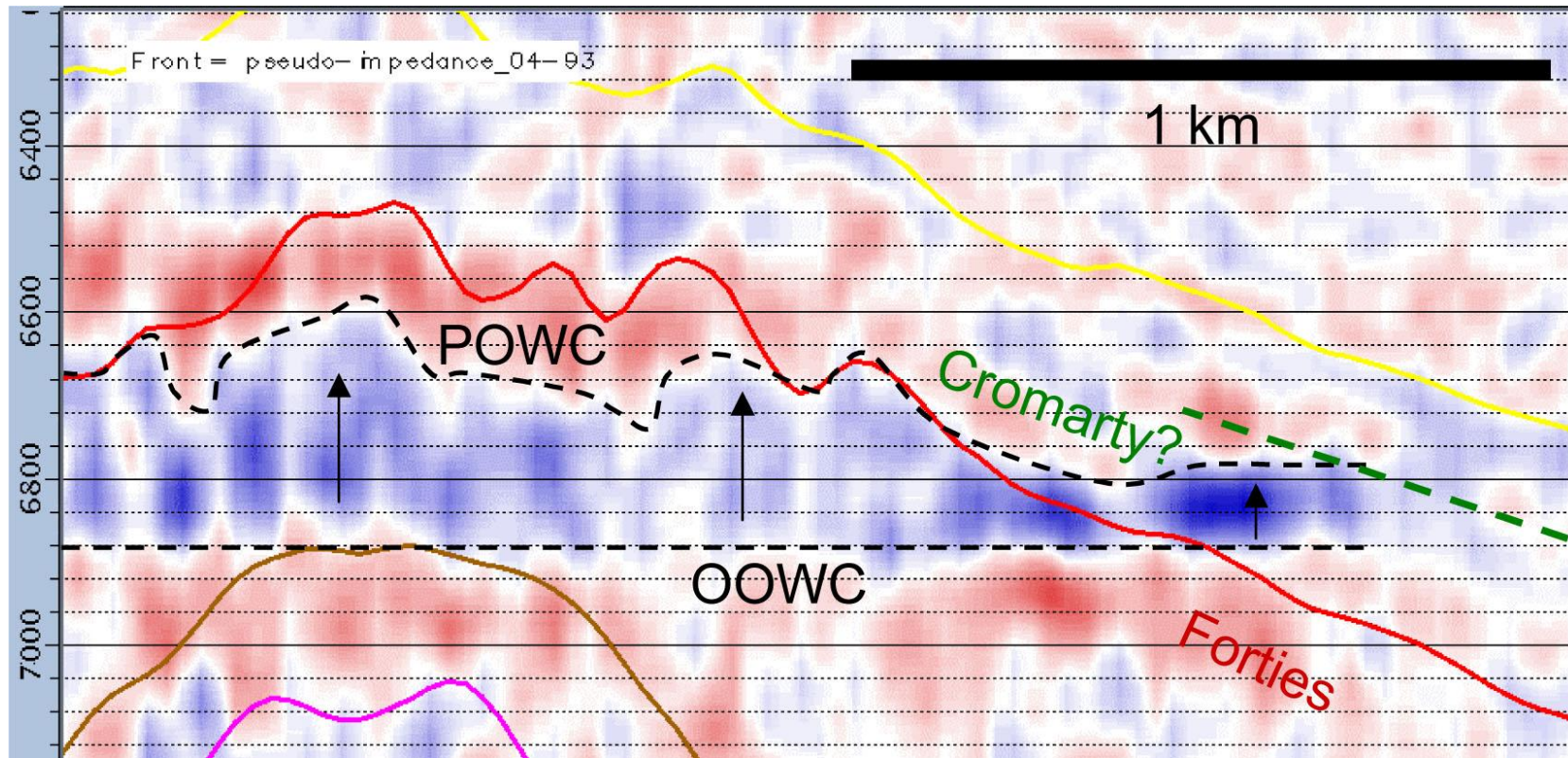
Figure 6. In the southeast of the field, (blue) aquifer influx (hardening) extends well outside the top Forties pick on the 2004-1993 difference cube, indicative of significant Cromarty presence, and connection with the Forties. (Note also the highly variable Forties POWC on this section, caused by significant radial faulting orthogonal to section).
