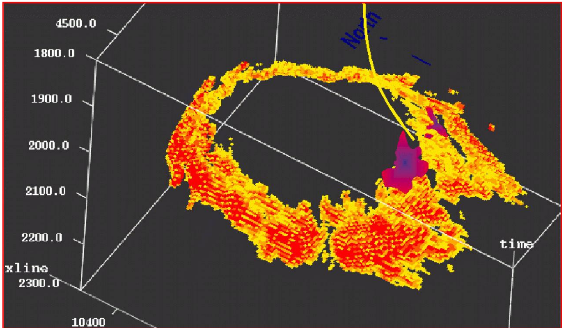
Figure 3. The main 4D hardening signal is shown for '98-'93 around the field (after Kloosterman et al, 2003).
