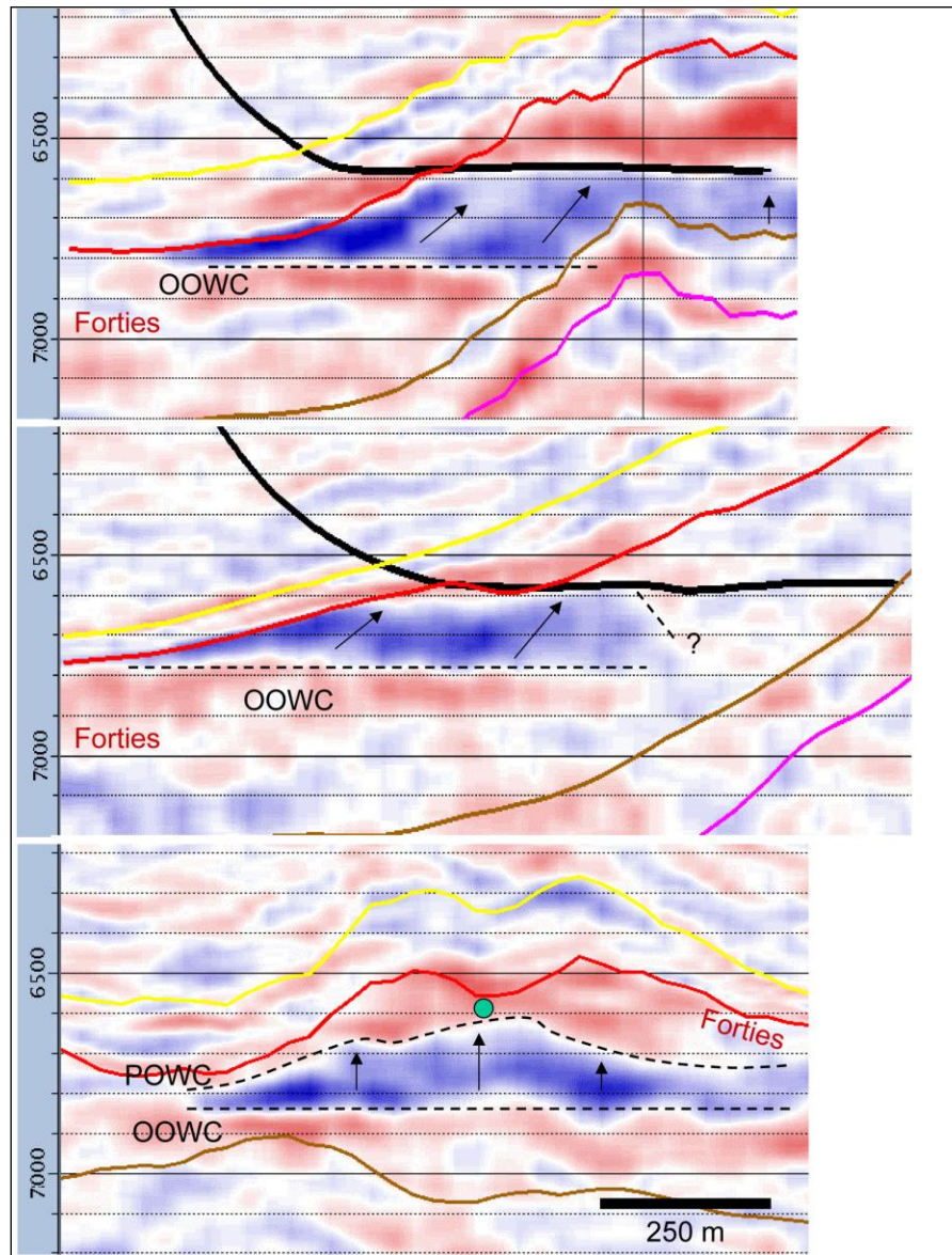
Figure 4. Different flood patterns at well seen on the 98-93 difference cube. Upper panel: water flood intersecting an entire well trajectory. Middle panel: water flood intersecting only the heel of a well. Lower panel: doming orthogonal to a well (green circle).
