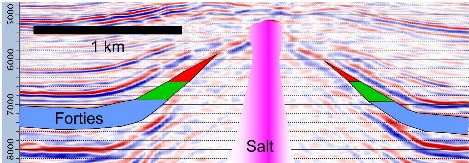
Figure 1. West-east cross section across the northern part of Gannet C showing pre-production fluid distribution in the Forties and approximate salt structure. All figure depths in ft. (No vertical exaggeration on this figure).
