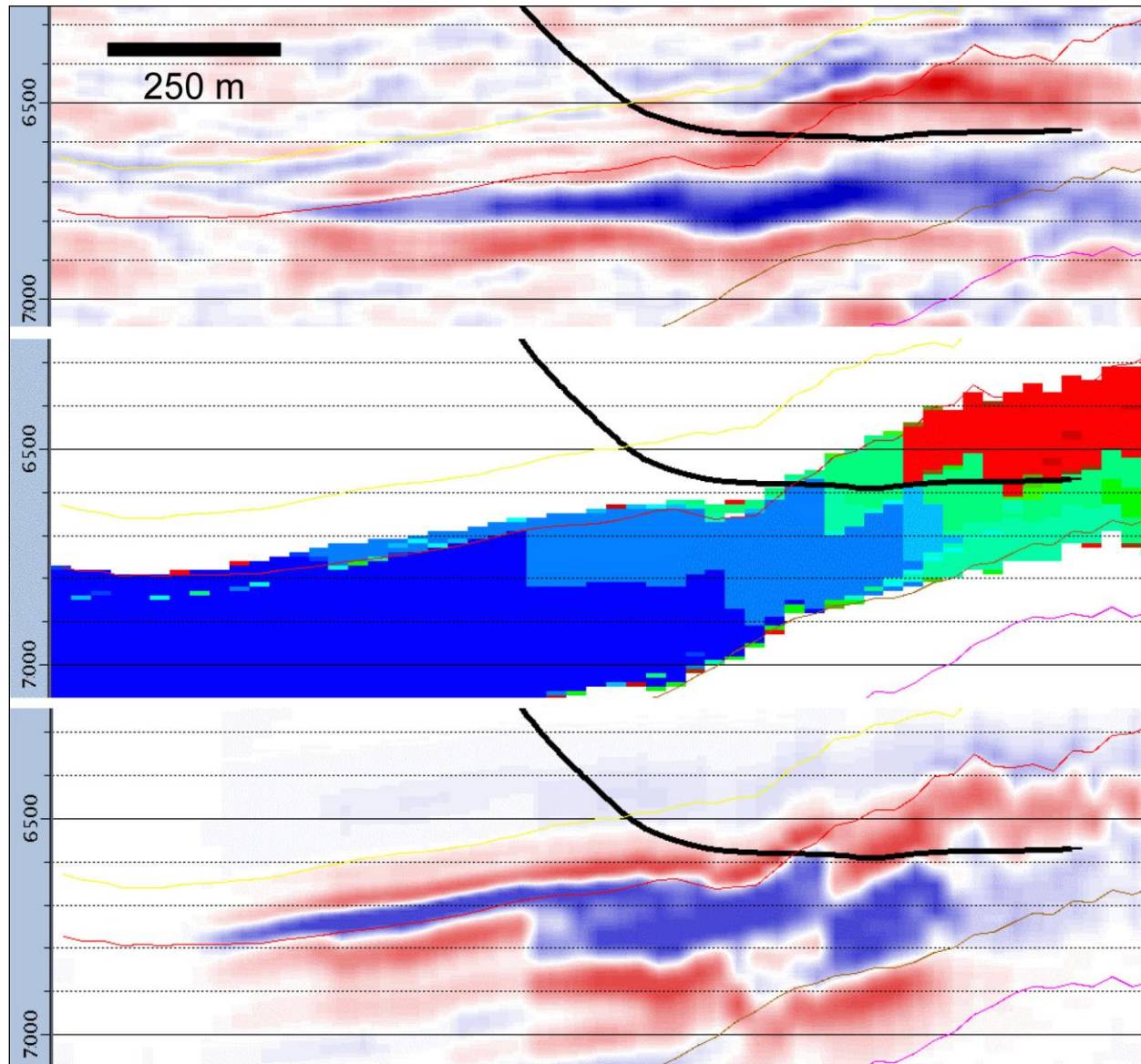
Figure 7. A comparison '98-'93 difference seismic (upper panel), simulation saturations from '98 (middle panel), and the corresponding simulator difference synthetic ('98-'93) during seismic history matching. In this case, the model is showing too much water sweep below the heel of the well and too little water sweep below the toe of the well, compared with the real seismic which shows a more uniform sweep pattern.
