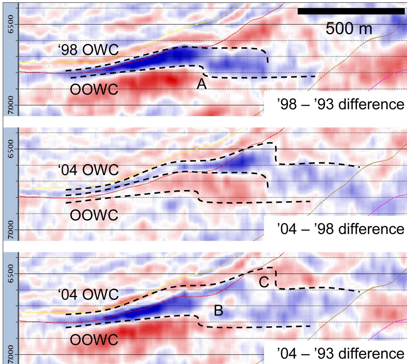
Figure 2. Interpreting contacts on pseudo-impedance difference cubes. The upper two sections represent incremental time-steps, whilst the lowest one represents the whole time period.
