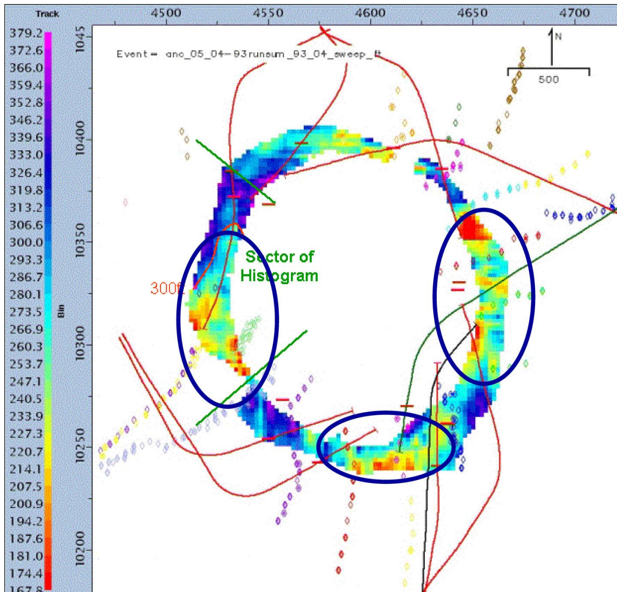
Figure 8. Map of Forties sweep thickness (feet) derived from 2004-1993 4D difference seismic, indicating the injector to producer workover area (south), and the two infill well targets (west and east).
