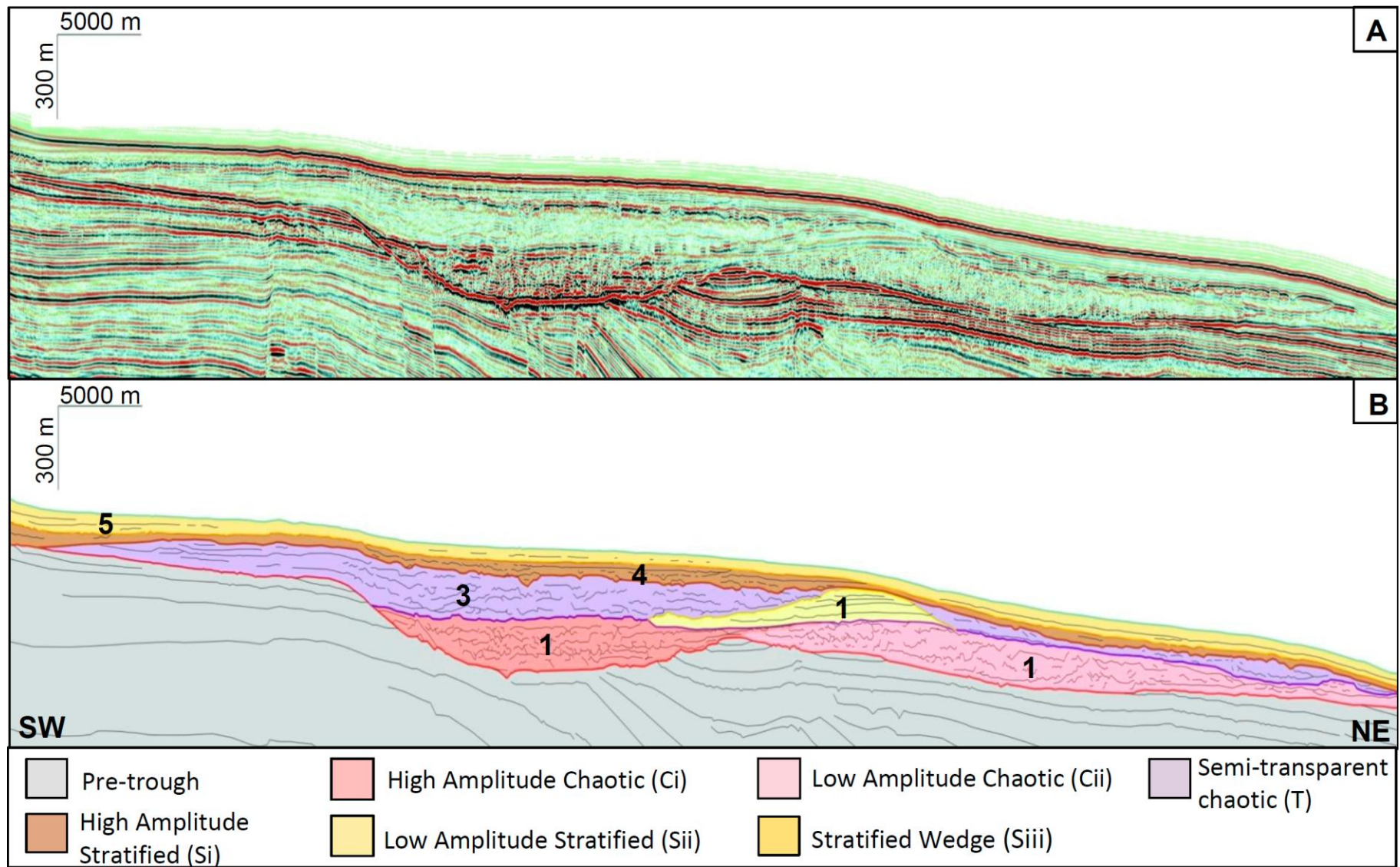
Figure 1. (A) Section of a seismic dip line through the Mackenzie Trough; (B) Schematic line drawing, illustrating the distribution of some of the seismic facies and sequences within the Mackenzie Trough.
