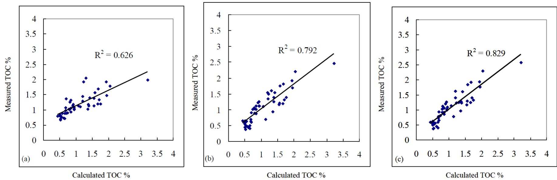
Figure 4. Calculated TOC vs. measured TOC (a for \Delta \log R technique; b for optimal superposition coefficient \Delta \log R technique; c for CARBOLOG technique).
