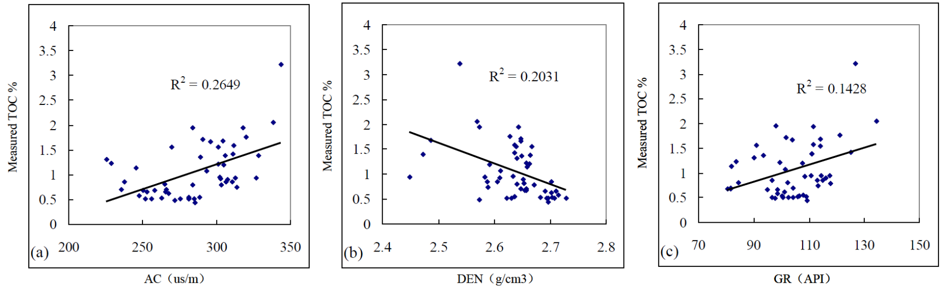
Figure 2. (a) Plot of sonic versus measured TOC; (b) plot of bulk density versus measured TOC; (c) Plot of natural gamma ray versus measured TOC.
