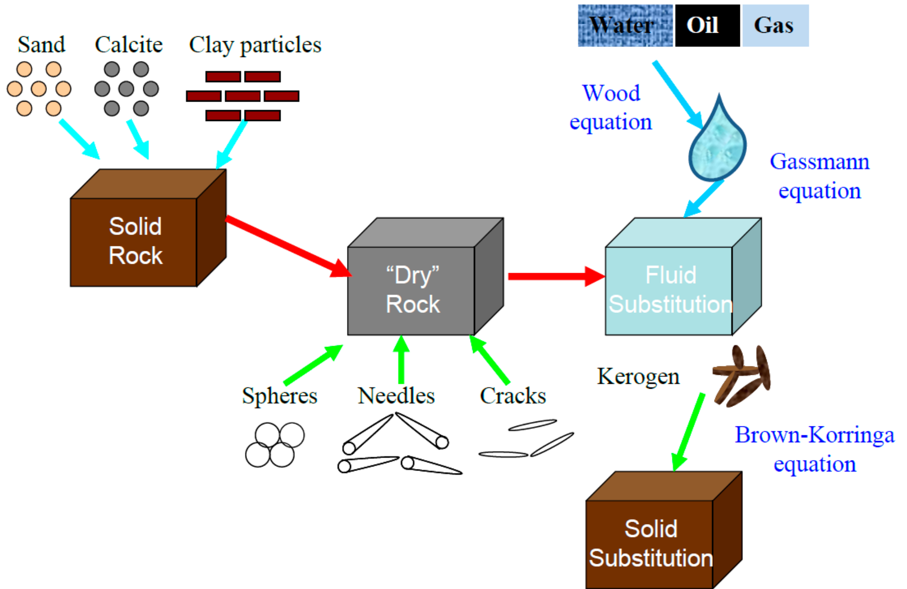
Figure 5. Schematic view of 3D SCA_DEM rock physics model for organic-rich shale.
