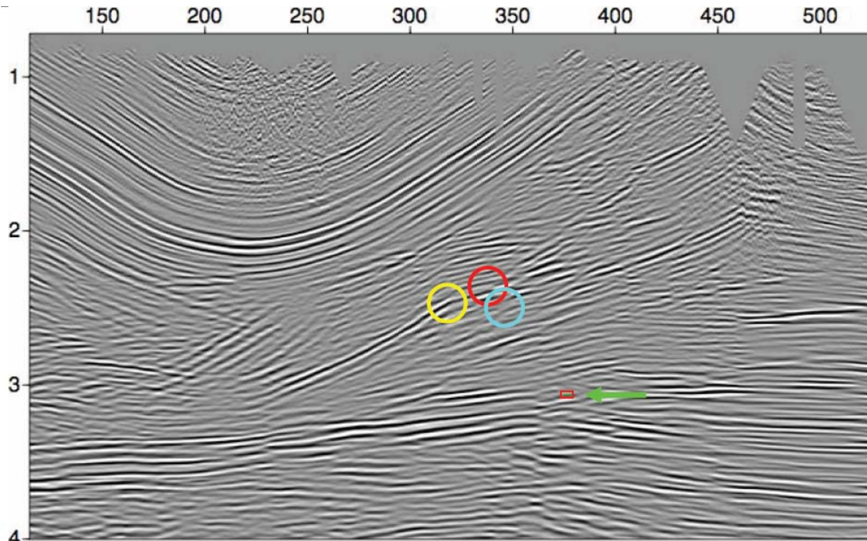
Figure 5. Inline slice from poststack time migration. The green marker represents the position that the well intersected the target horizon. The circles show the position of a fold on a reflector as it appears on the time section (yellow), the isotropic depth section (blue), and the anisotropic depth section (red).
