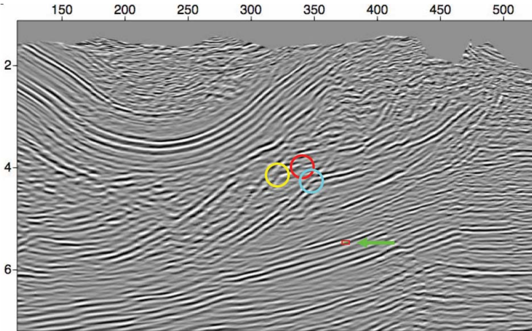
Figure 6. Inline slice from a previous isotropic depth migration project. The green marker represents the position that the well intersected the target horizon. The circles show the position of a fold on a reflector as it appears on the time section (yellow), the isotropic depth section (blue), and the anisotropic depth section (red).
