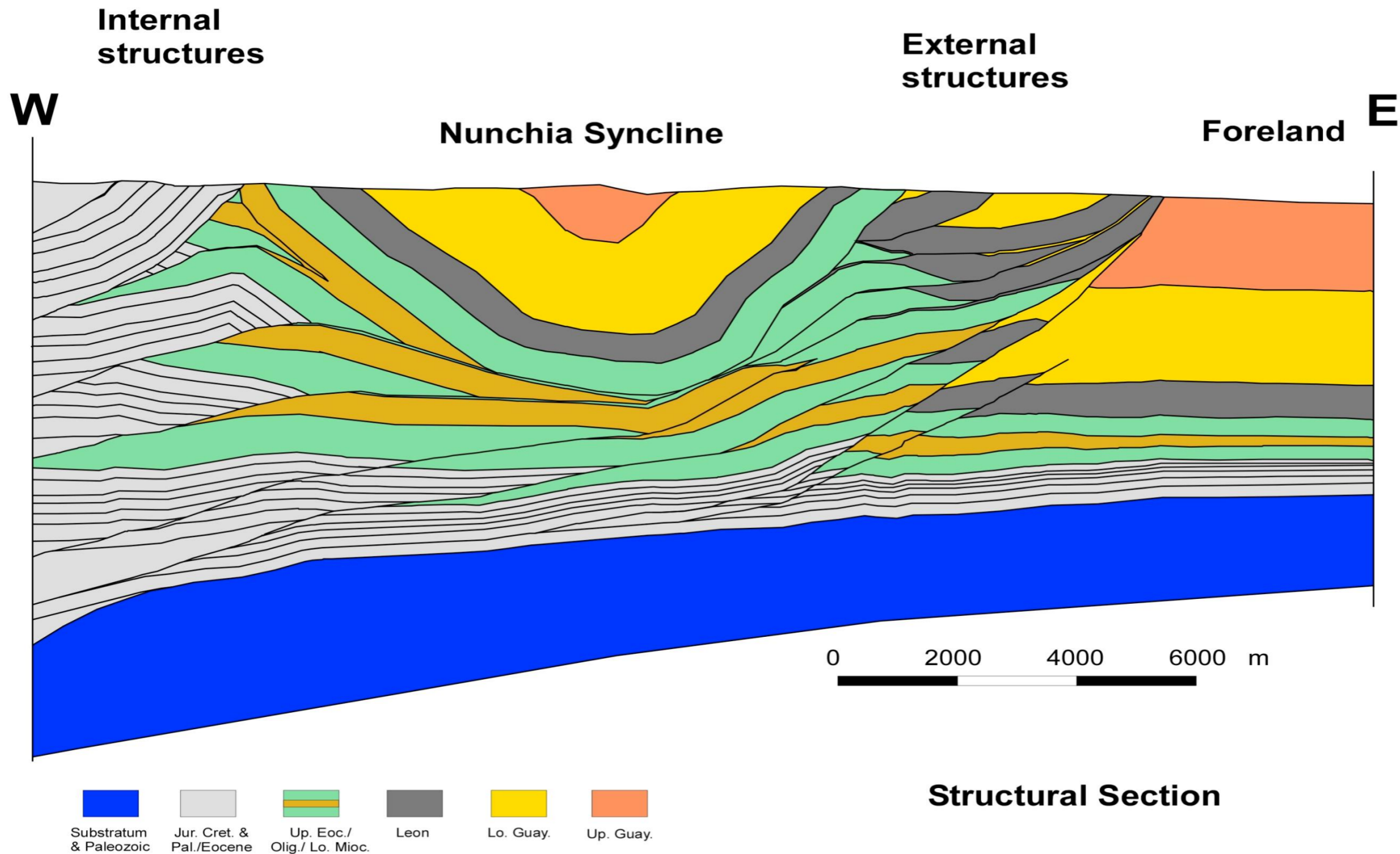
Figure 3. Schematic Structural Section: The foothills belt in the area can be separated into 4 areas as described with details by Rochat et al, 2003: Internal Structures in the western part, Nunchia Syncline that extends widely in the area and External Structures next to the western limit of the Foreland (figure from Rochat et al, 2003).
