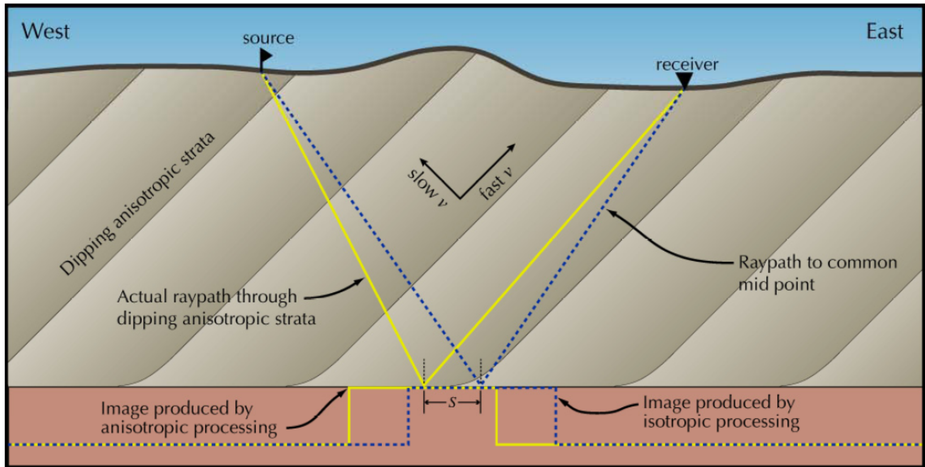
Figure 2. Cross-section showing lateral movement predicted from isotropic processing of data where transverse isotropy with a tilted axis of symmetry is present. The dashed lines represent the result of isotropic processing. S is the distance between the actual subsurface reflection point and the reflection point when the processing algorithm assumes isotropy (modified from Vestrum et al, 1999).
