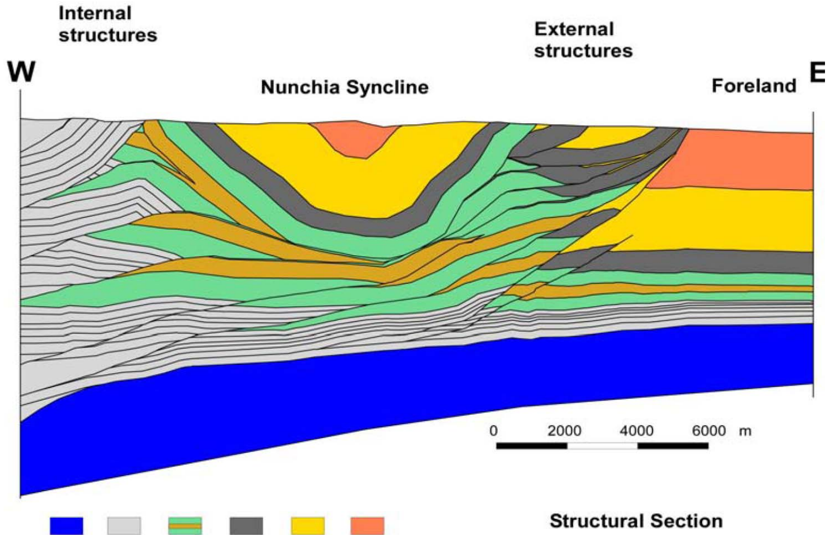
Figure 3. Schematic structural section. The foothills belt in the area can be separated into 4 areas as described with details by Rochat et al. (2003): Internal Structures in the western part, Nunchia Syncline that extends widely in the area and External Structures next to the western limit of the Foreland (from Rochat et al., 2003).
