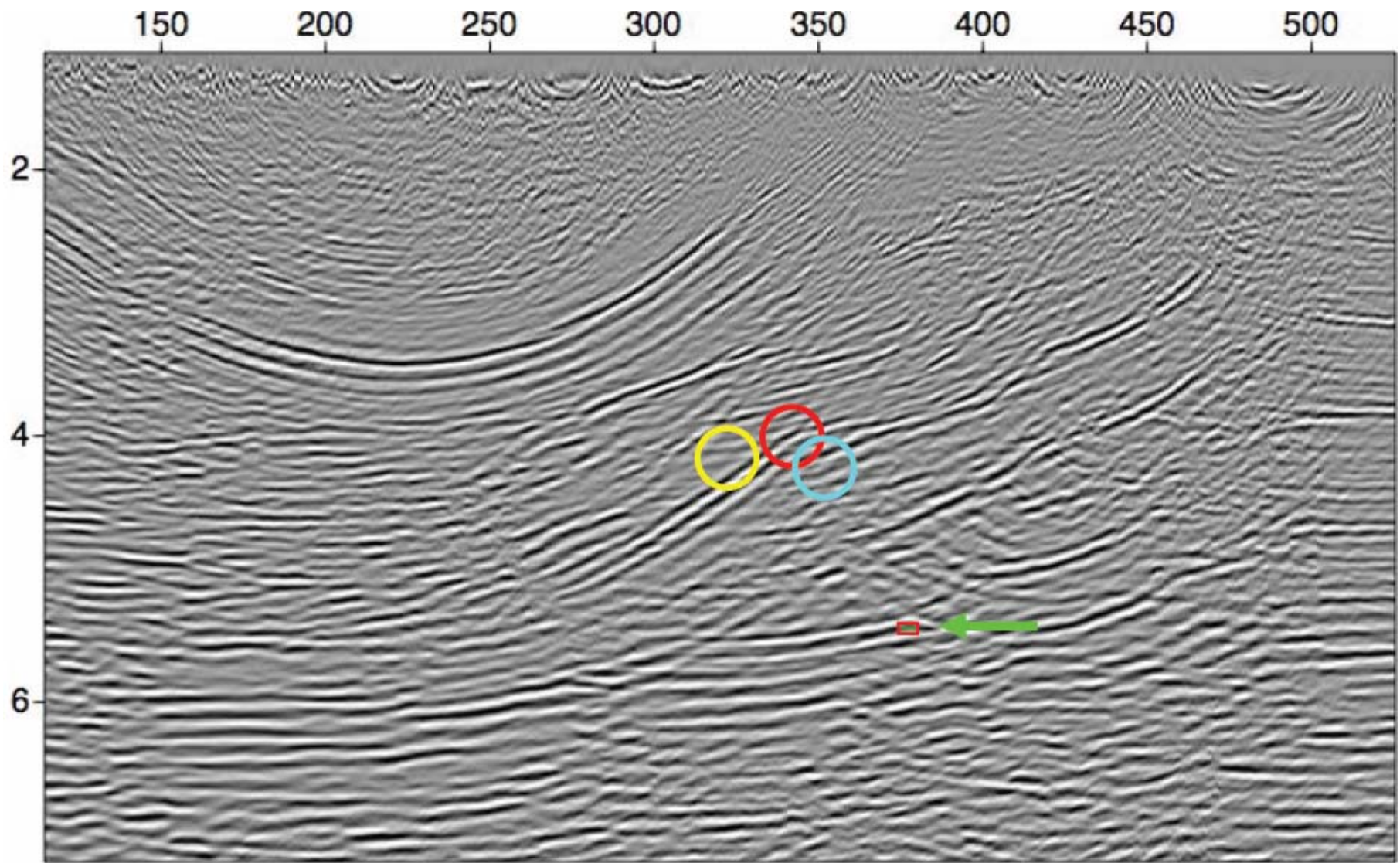
Figure 7. Inline slice from prestack anisotropic depth migration after 12 iterations of model building. The green marker represents the position that the well intersected the target horizon. The circles show the position of a fold on a reflector as it appears on the time section (yellow), the isotropic depth section (blue), and the anisotropic depth section (red).
