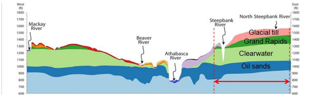
Figure 1. Conceptual geological model for the area. Readapted with permission from Chen et al., (2013)
