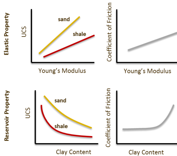
Figure 5. General trends of failure parameters as a function of elastic property and reservoir property (clay volume).
