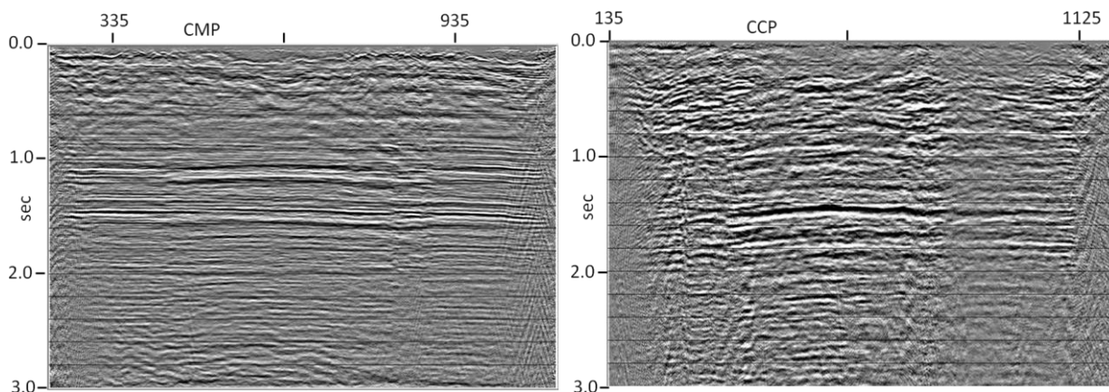
FIG. 2. Brute stacks of Hussar 3C survey, no statics applied. CMP stack of PP data on the left, CCP stack of PS data on the right.
