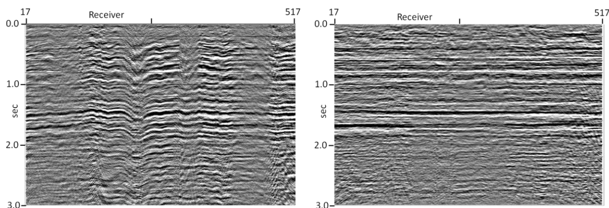
FIG. 5. Common-receiver stack of uncorrected Hussar PS data (left) strongly suggests non-stationary shear statics are required to correct the data. The common-receiver stack on the right shows the result of applying raypath interferometry, which applies non-stationary corrections without altering NMO velocities.
