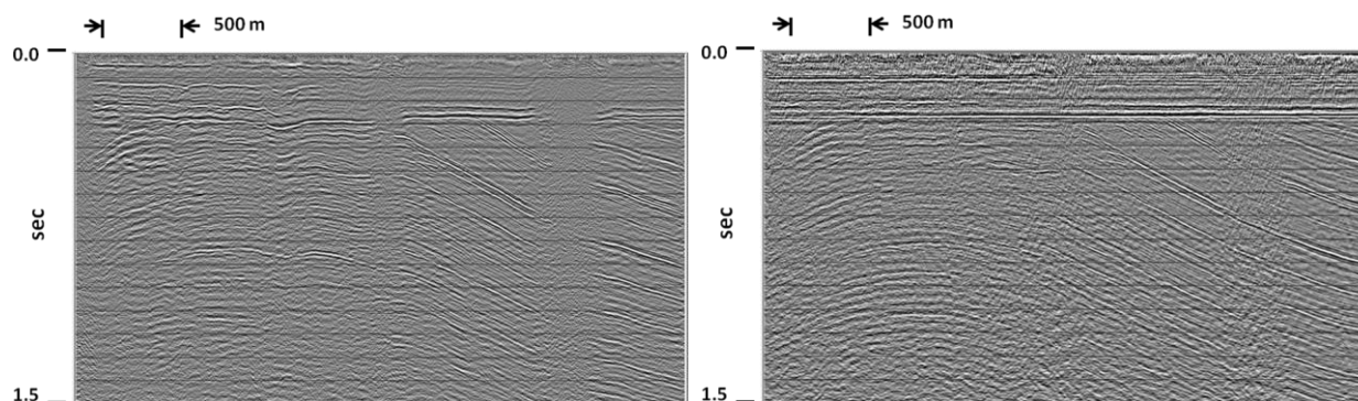
FIG. 1. MacKenzie Delta high-resolution line with visible statics on the brute CMP stack (left). The CMP stack on the right, after raypath interferometry, shows much more near-surface detail, as well as event continuity in the deep structure.
