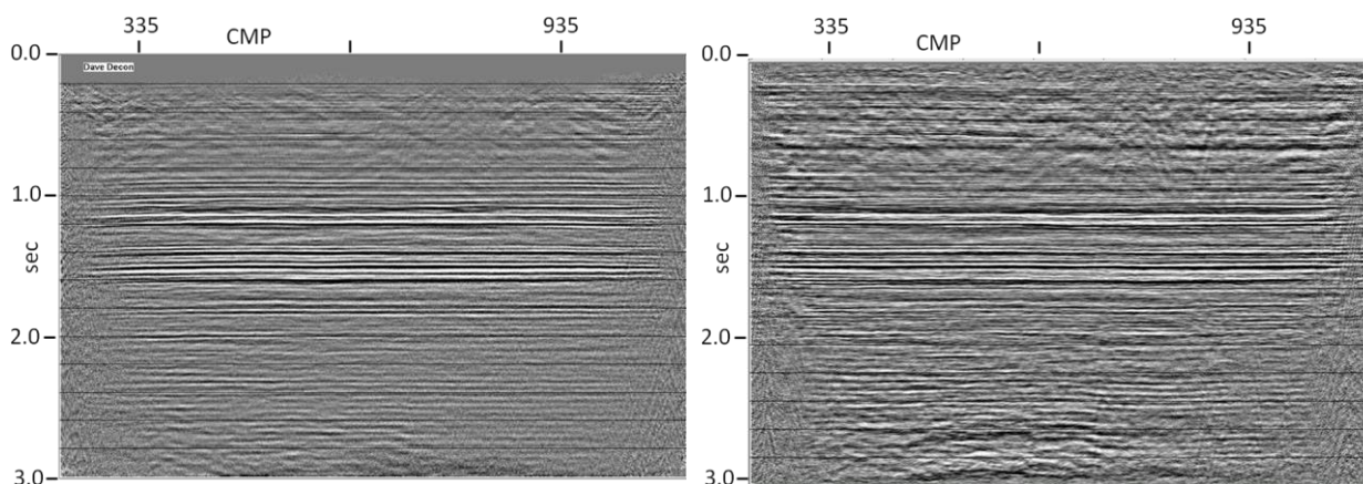
FIG. 3. Comparison of CMP stacks of Hussar PP data after conventional statics and NMO analysis (left) and after raypath interferometry with a single NMO function (right).
